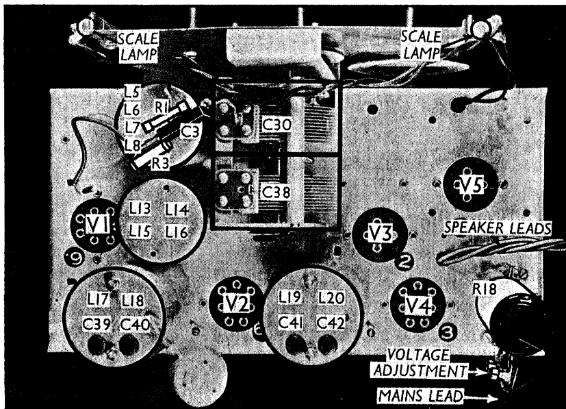
Plan view of the chassis. Note the components above the L5-L8 coil unit.
