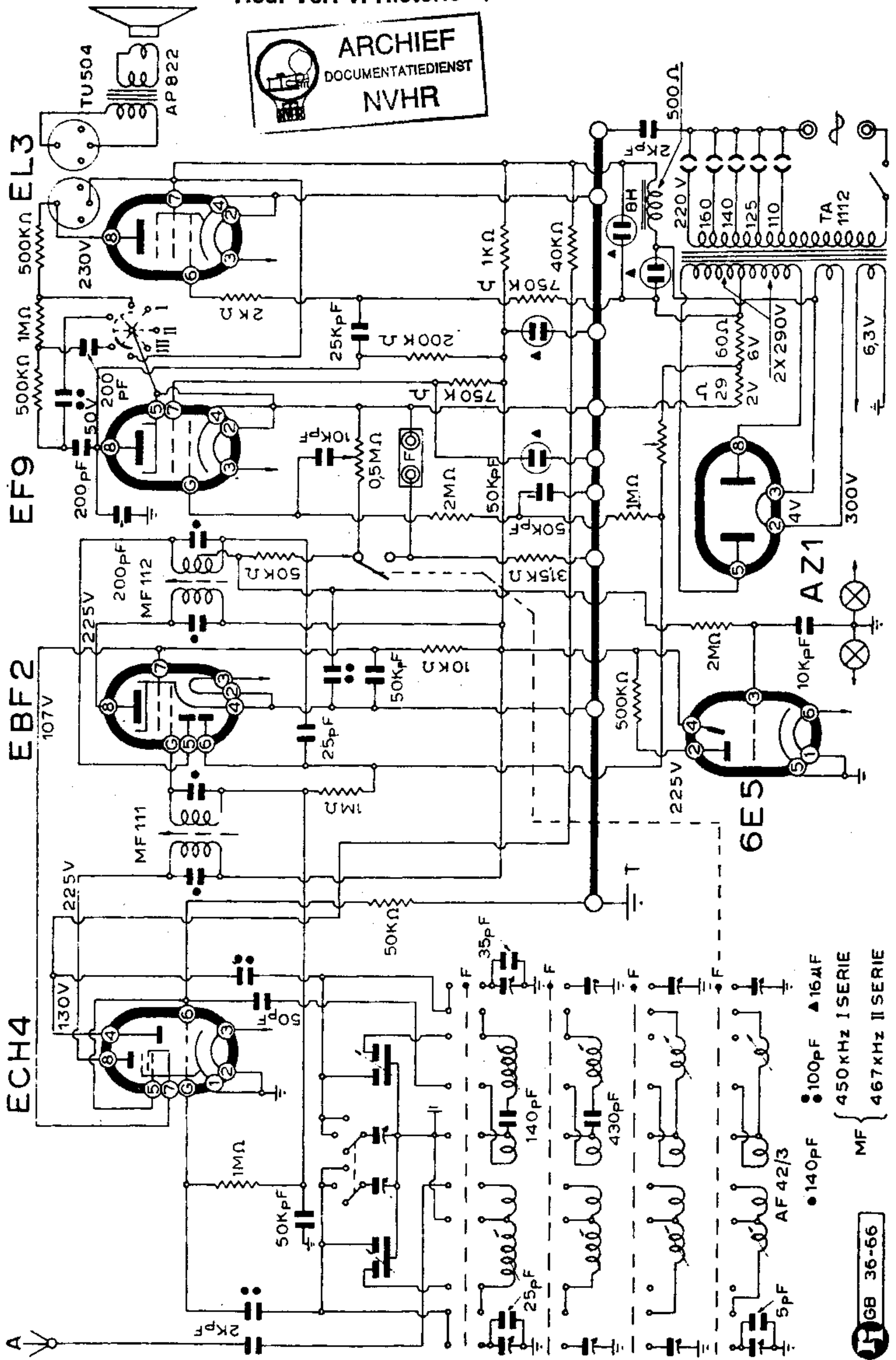
UNDA RADIO - Mod. Super Quadri Unda R 64/5
