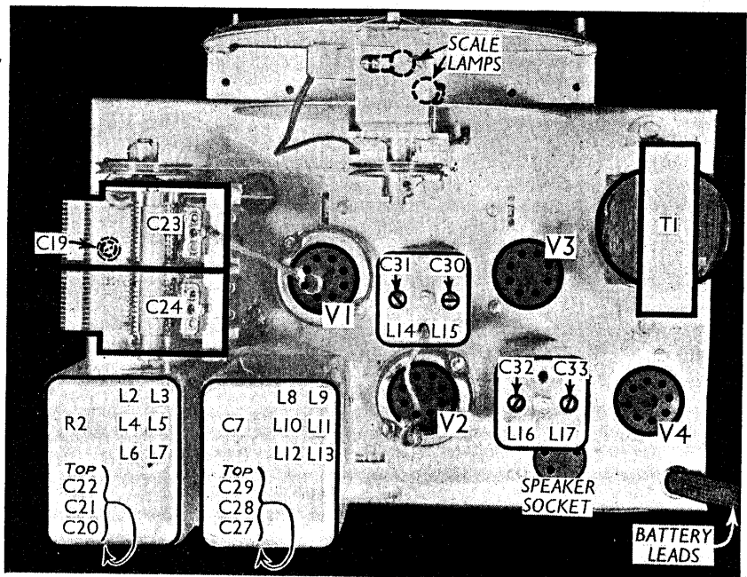
Plan view of the chassis. The trimmers in the large coil units are numbered from top to bottom.
