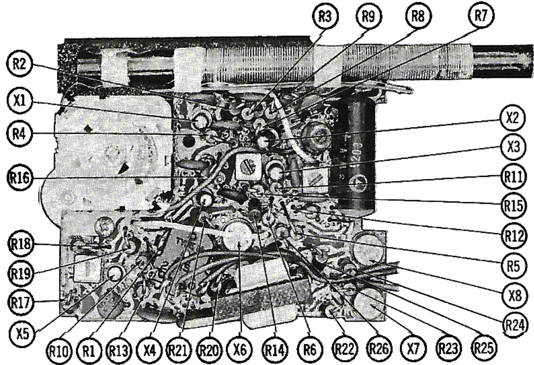
CHASSIS TOP VIEW - RESISTOR & TRANSISTOR IDENT.
