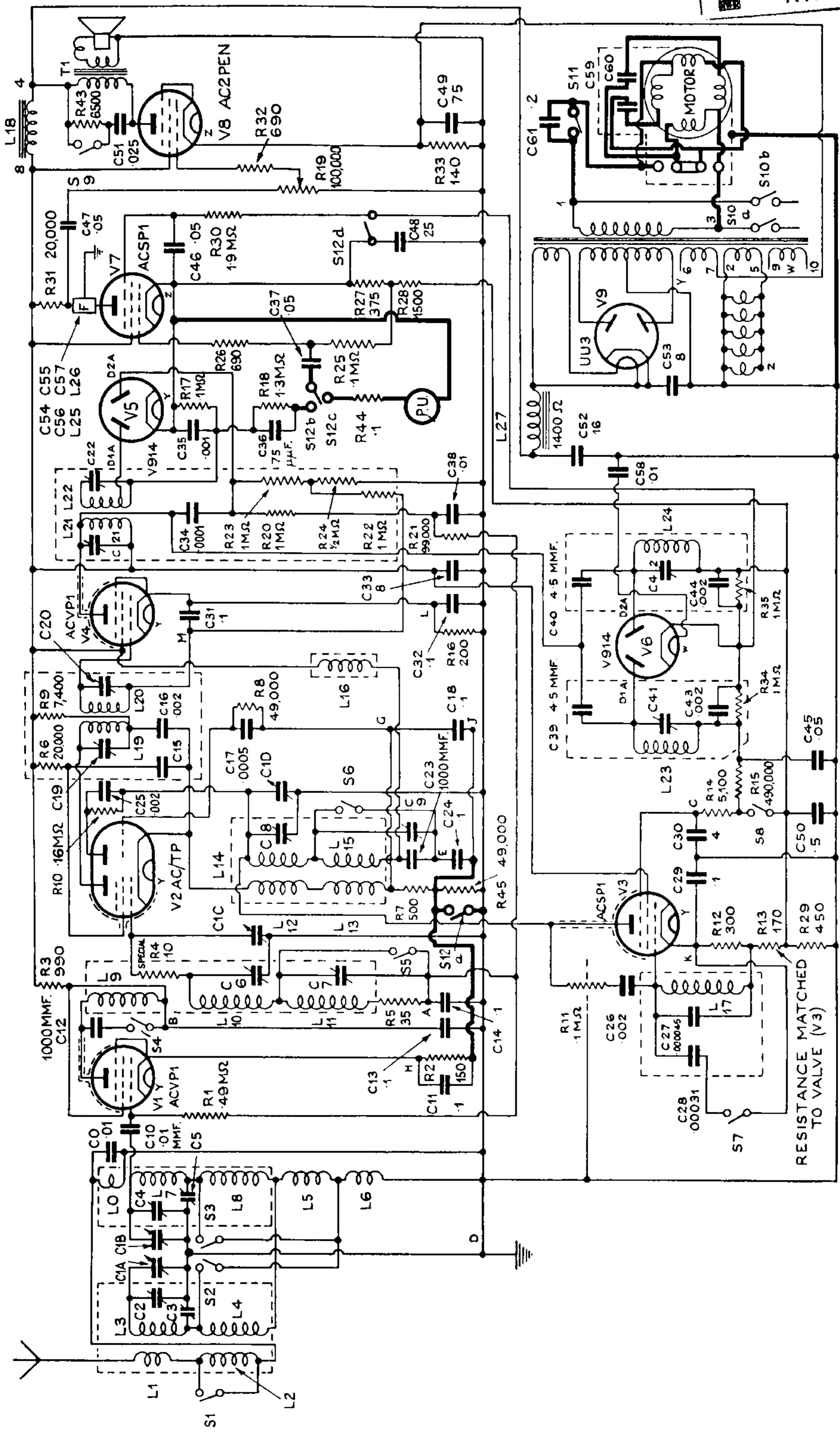
A28RG CIRCUIT DIAGRAM
