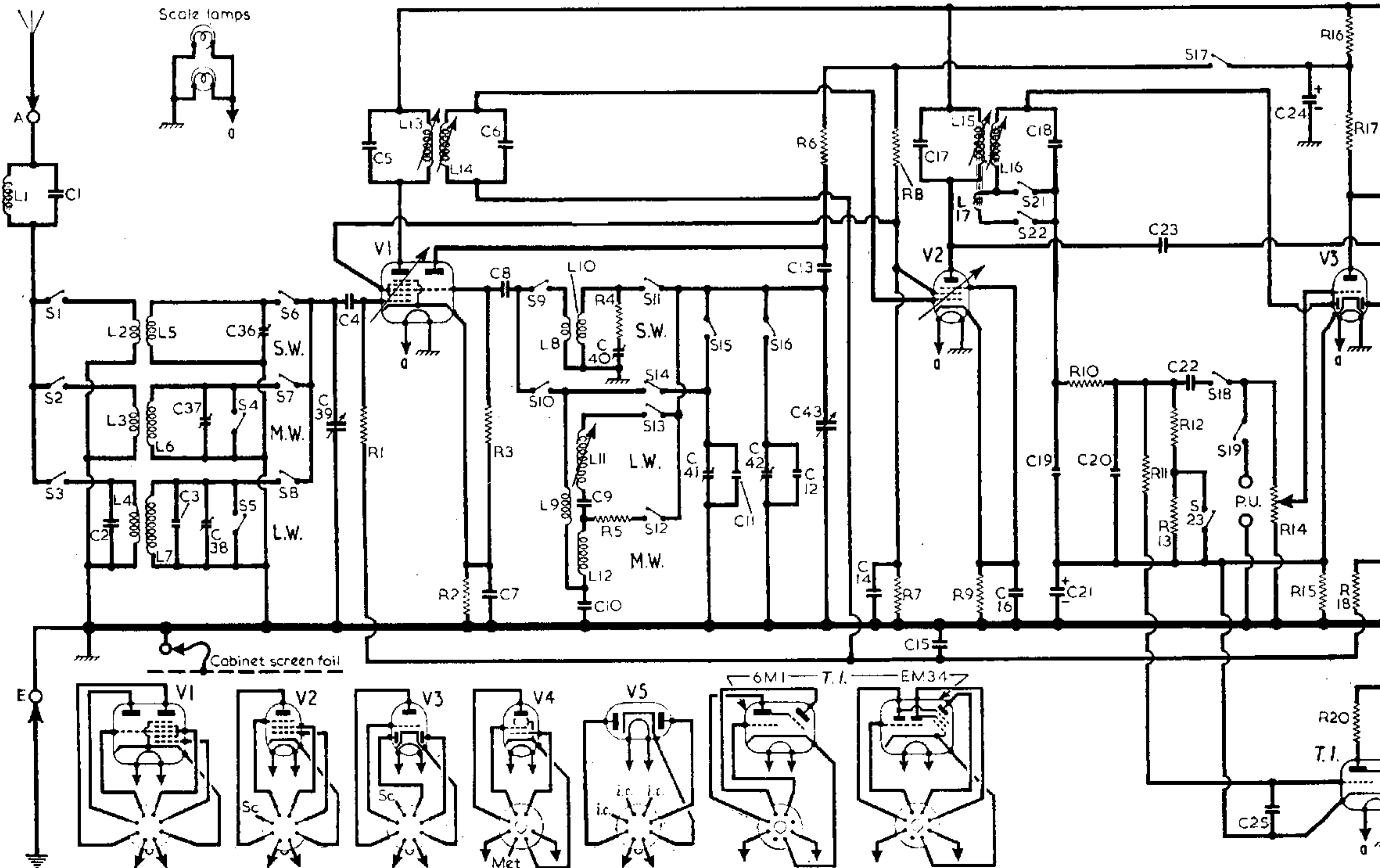
Circuit diagram of the Murphy A170 receiver, as produced at Welwyn. Another version, produced at Dublin, contains two small diodes which are explained overleaf under "Modifications". The temperature fuse in the mains transformer circuit melts if the transformer over-
