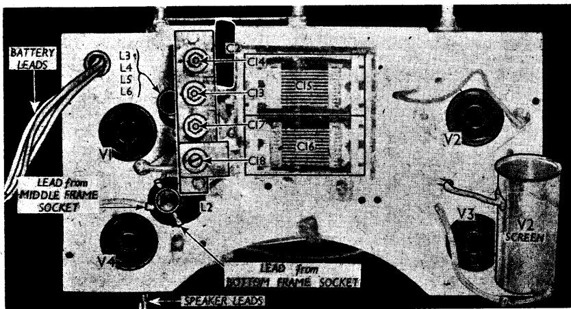
Plan view of the chassis. All the RF and oscillator coils and trimmers, with the exception of L1, are shown here. The connections to L1 are indicated.
