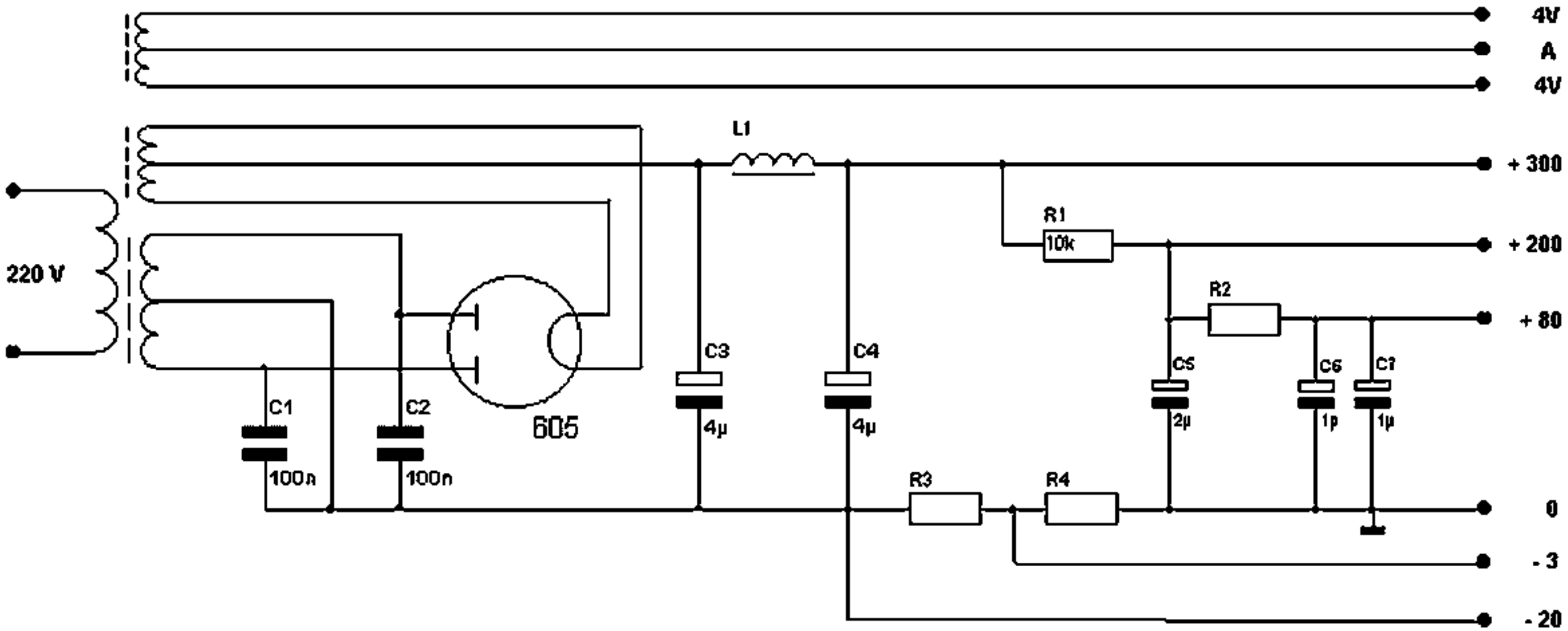
Power supply KRO PAN Europa
