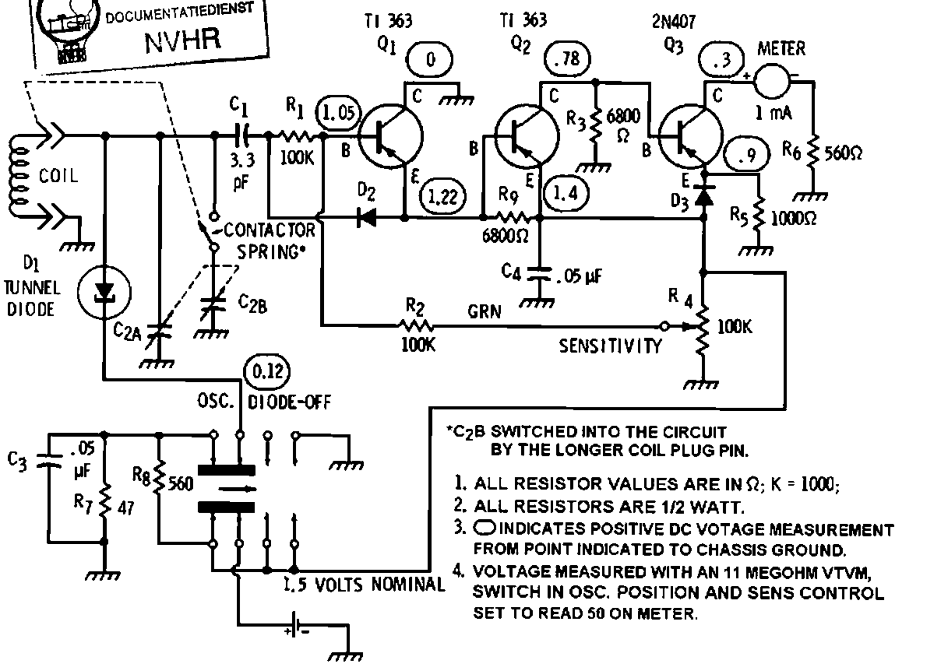
SCHMATIC OF THE HEATHKIT TUNNEL DIPPER MODEL HM-10A
