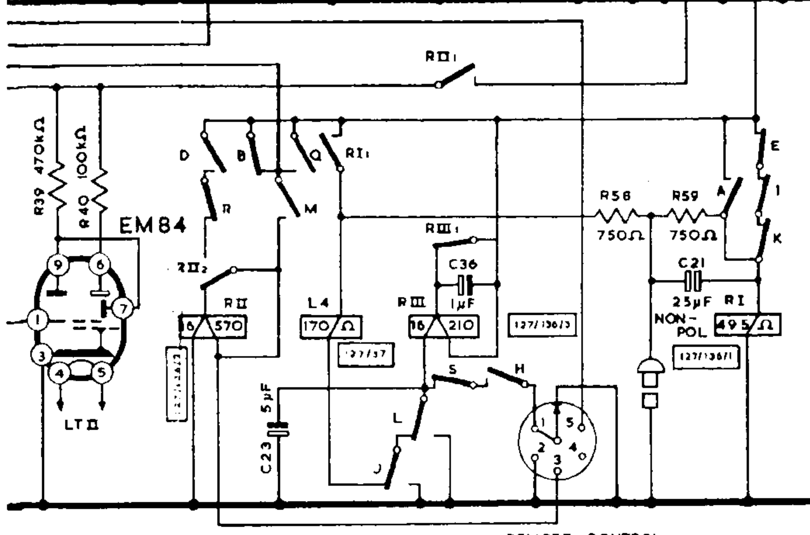
REMOTE CONTROL
