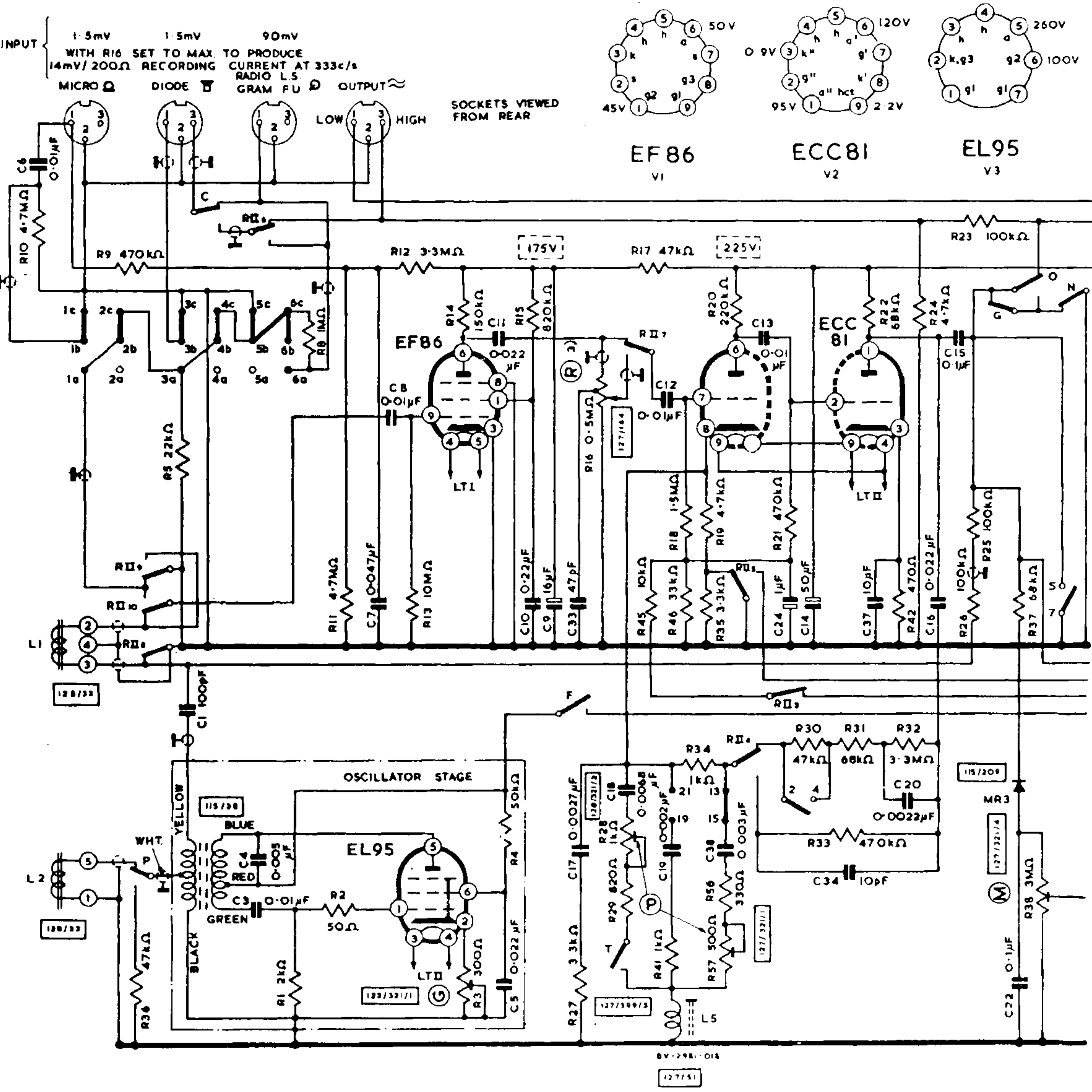
CIRCUIT DIAGRAM—
