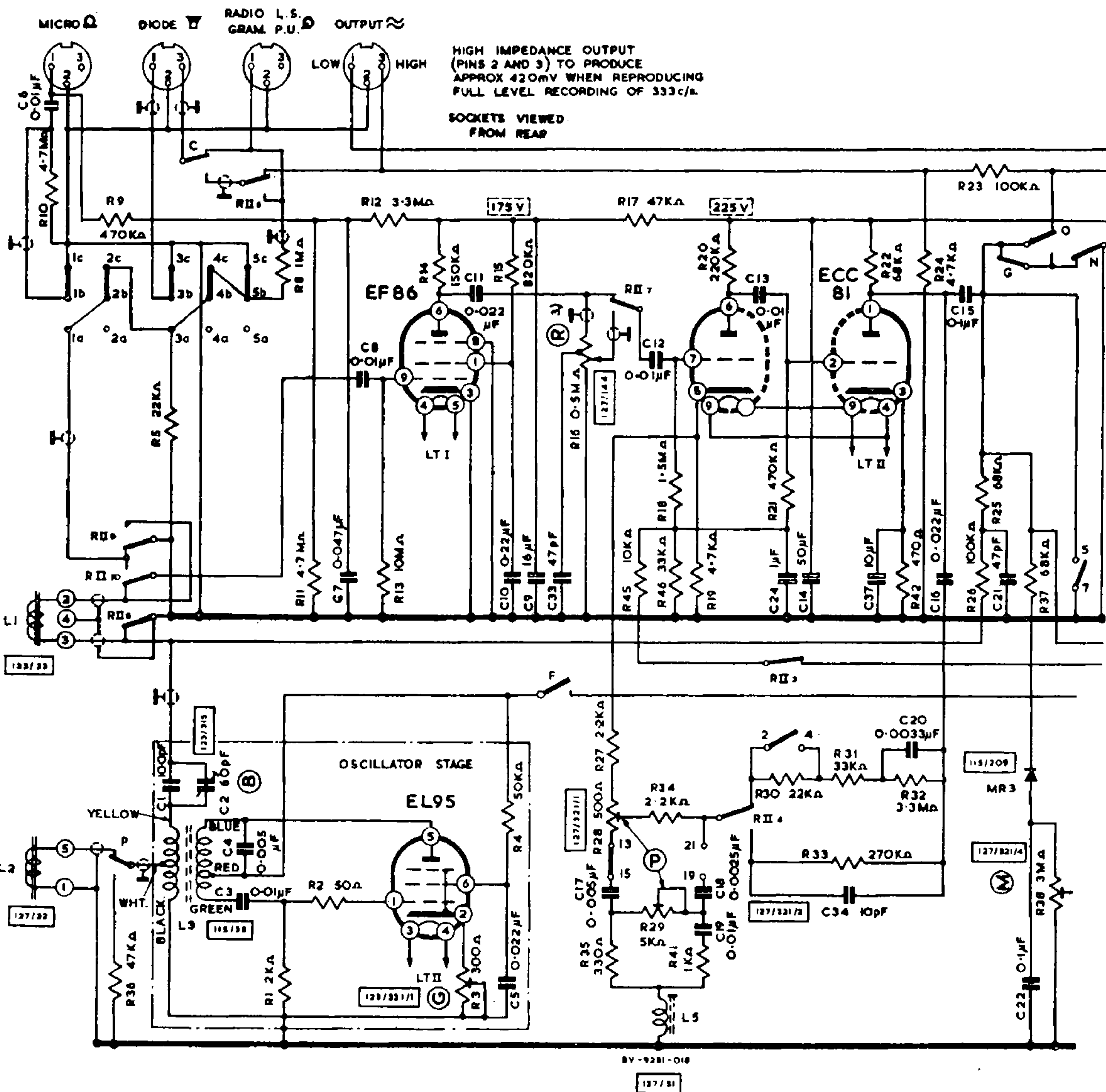
CIRCUIT DIAGRAM—
