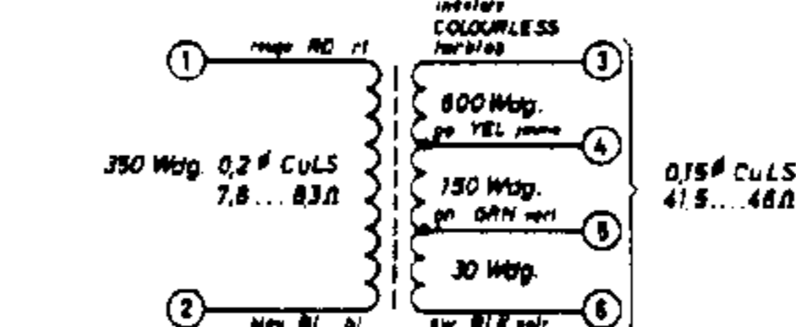
HF-Generatorspule HF GENERATOR COIL Bobine Generateur HF BV 9281—086 (TK 14 L)
