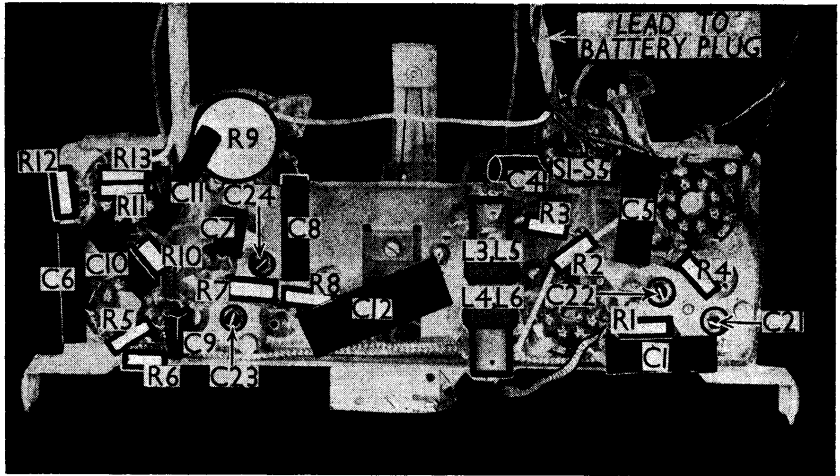
Under-chassis view. The switch unit is shown in detail in col. 1. Note the adjusting screws of the four IF trimmers, C21—C24.
