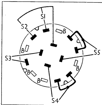
Diagram of the switch unit, looking at the underside of the chassis.
