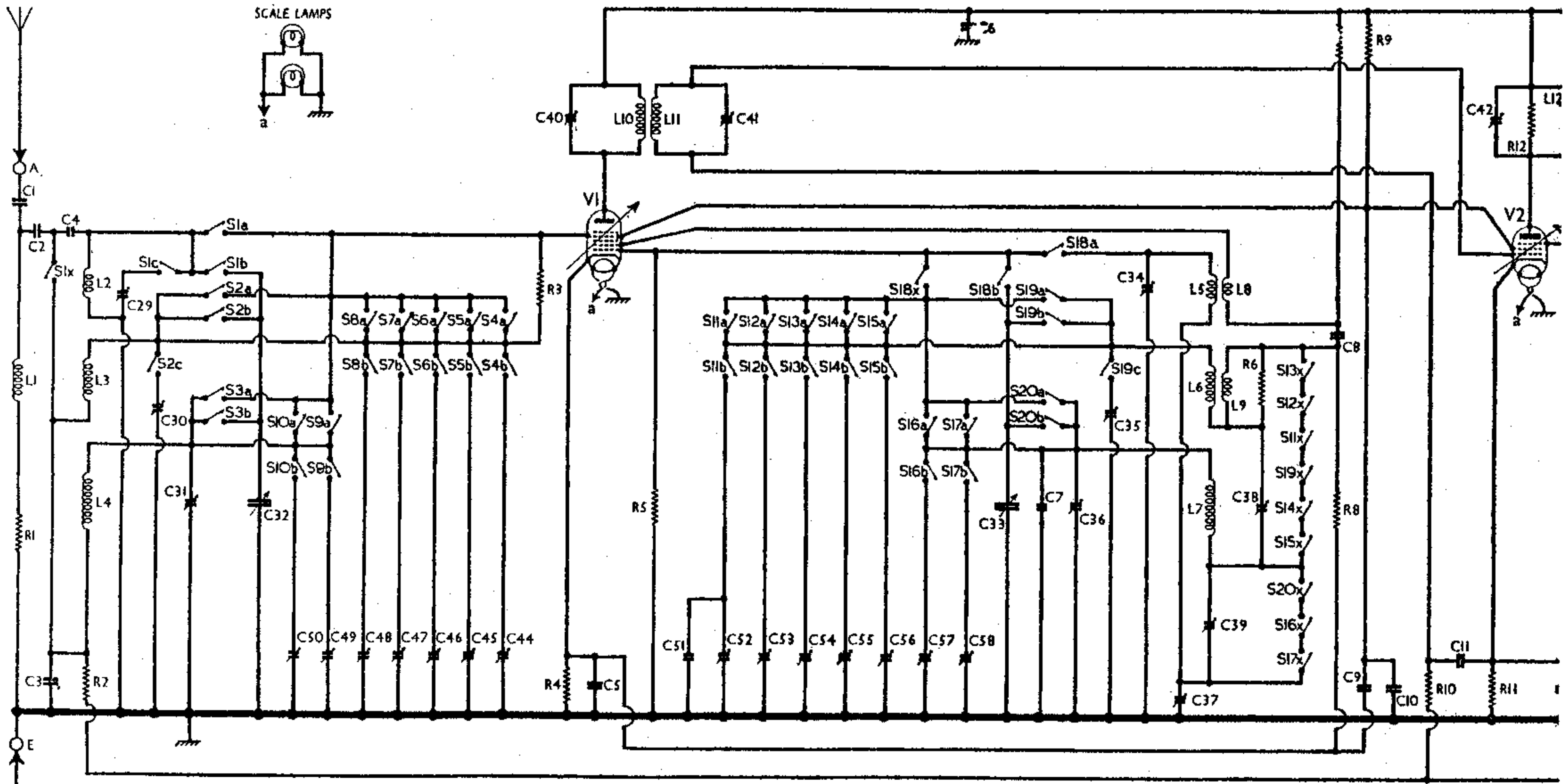
Circuit diagram of the Ferguson 771 table and 774 console "Pressabutton" superhets. All the switches with the exception of S22 are press-button operated, and they are code-numbered in the diagram to show their action. The coding is fully explained at the beginning of "Circuit Description." Differences in early models are described under "Chassis Divergencies" overleaf.
