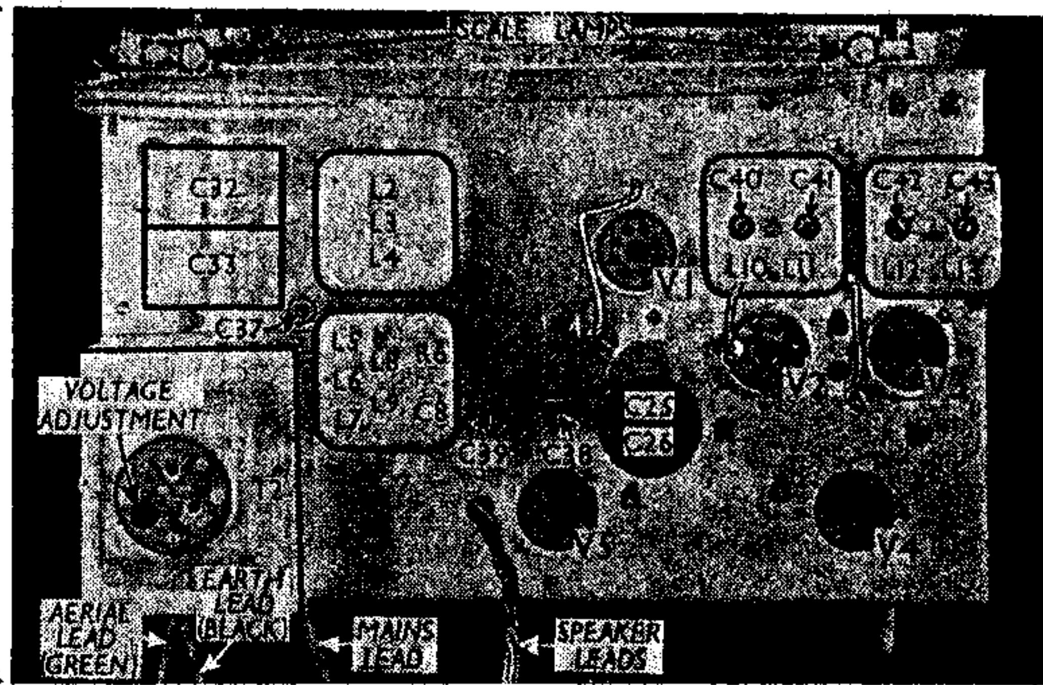
Plan view of the chassis. The tracker adjustments are indicated. R6 and C8 are inside the L5-L9 coil unit screen.
