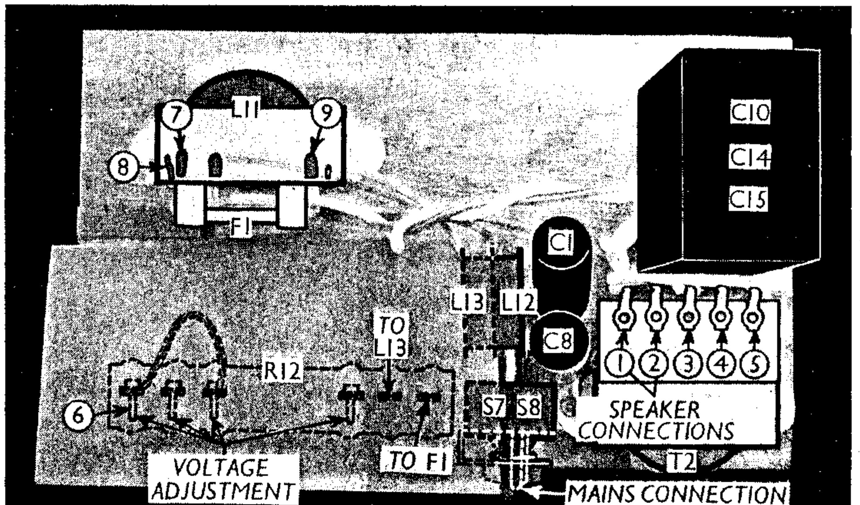
Plan view of the power unit. Connection points are numbered to agree with those in the under-chassis view.
