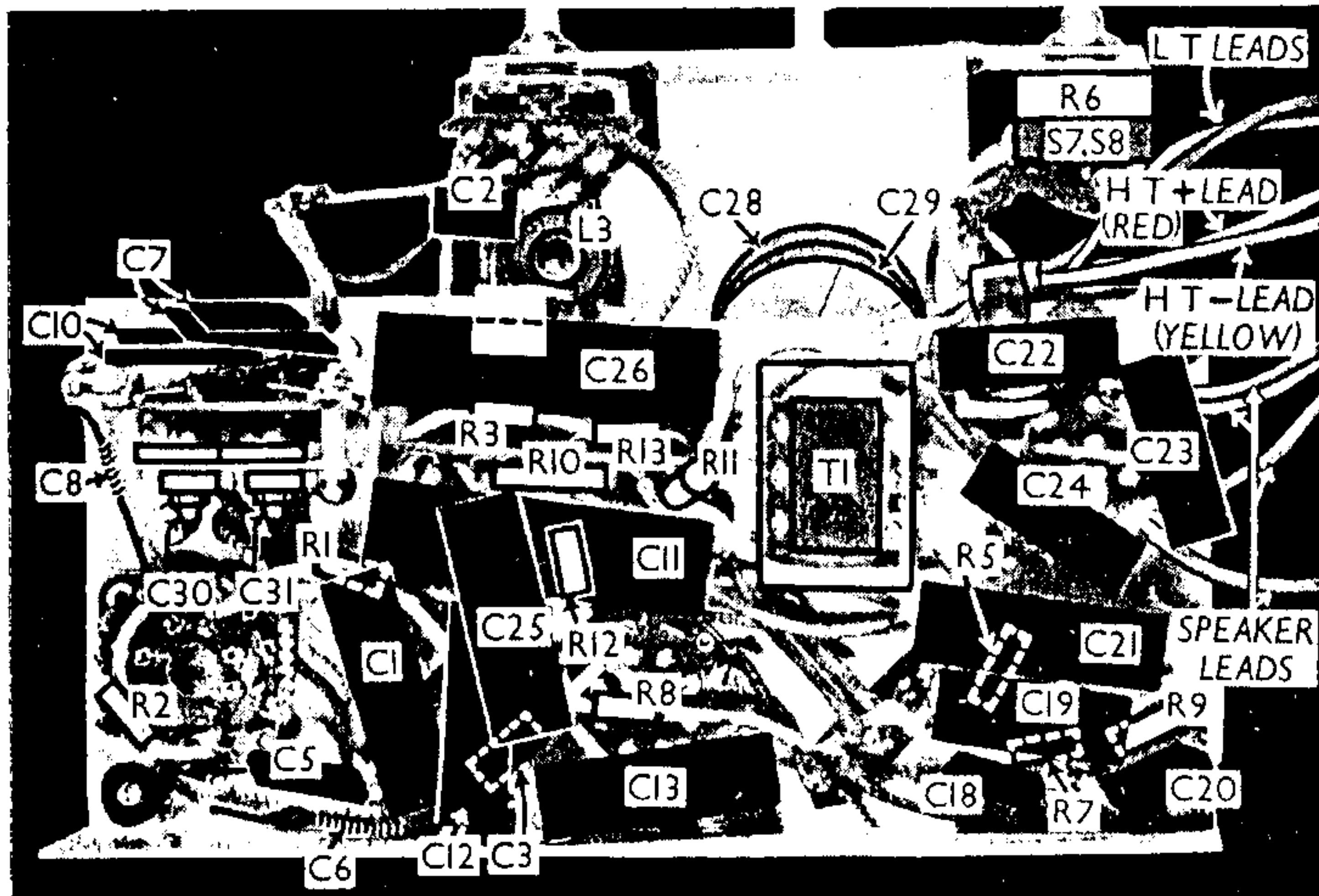
Under-chassis view, with various leads indicated.
