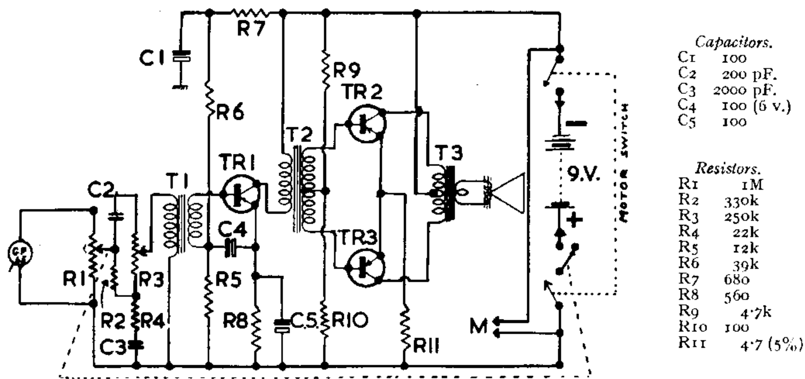
CIRCUIT DIAGRAM—DANSETTE "DIPLOMAT" Ned. Ver. v. Historie v/d Ra
