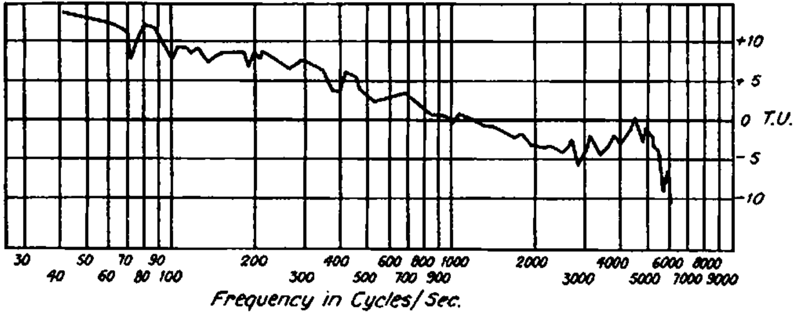
Average characteristic of B.T.H. Senior de Luxe Pick-up with volume control.
