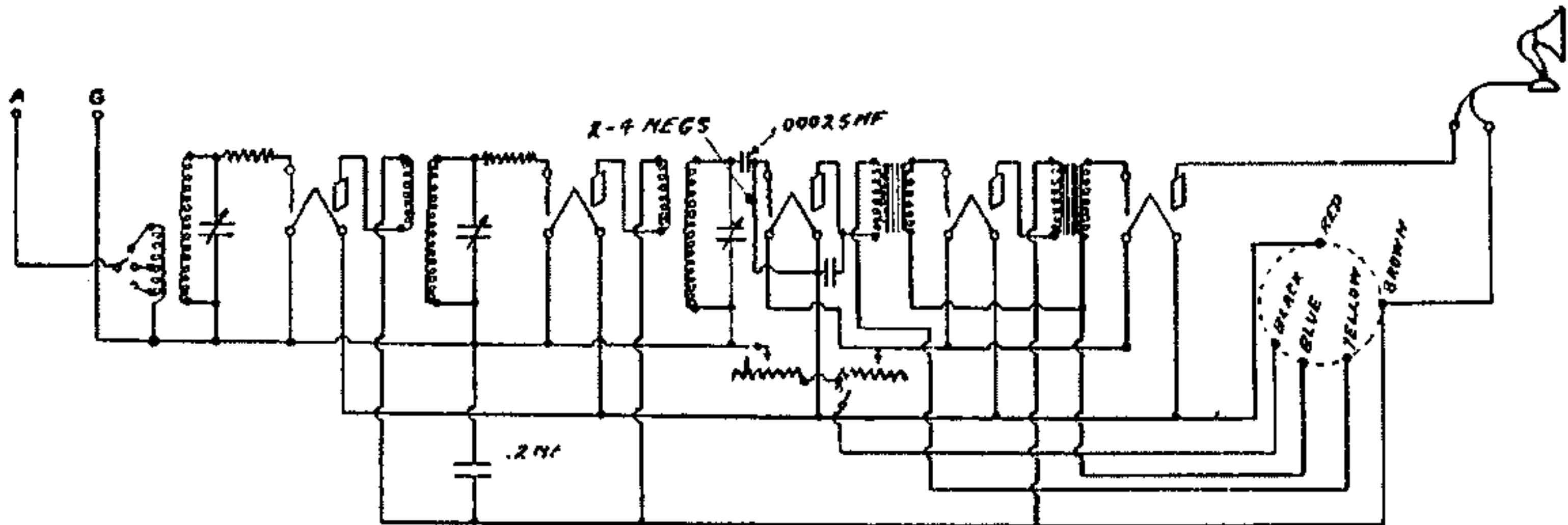
MODEL 21 DRY CELL SET No. 7780. WIRING DIAGRAM
