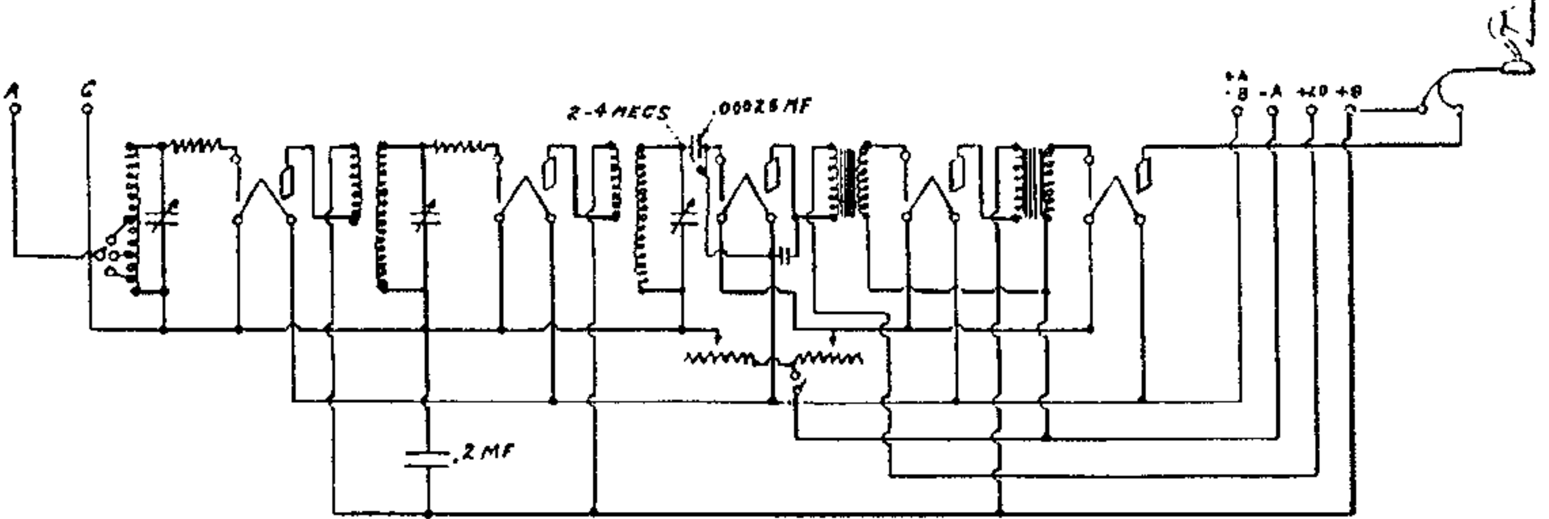
MODEL 20 SET No. 4640. WIRING DIAGRAM
