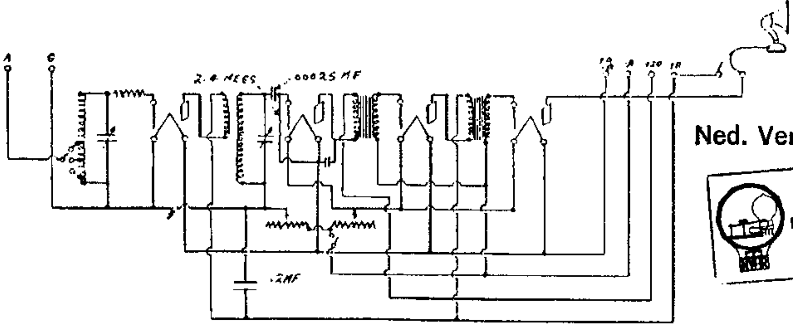
MODEL 19 SET No. 4880. WIRING DIAGRAM
