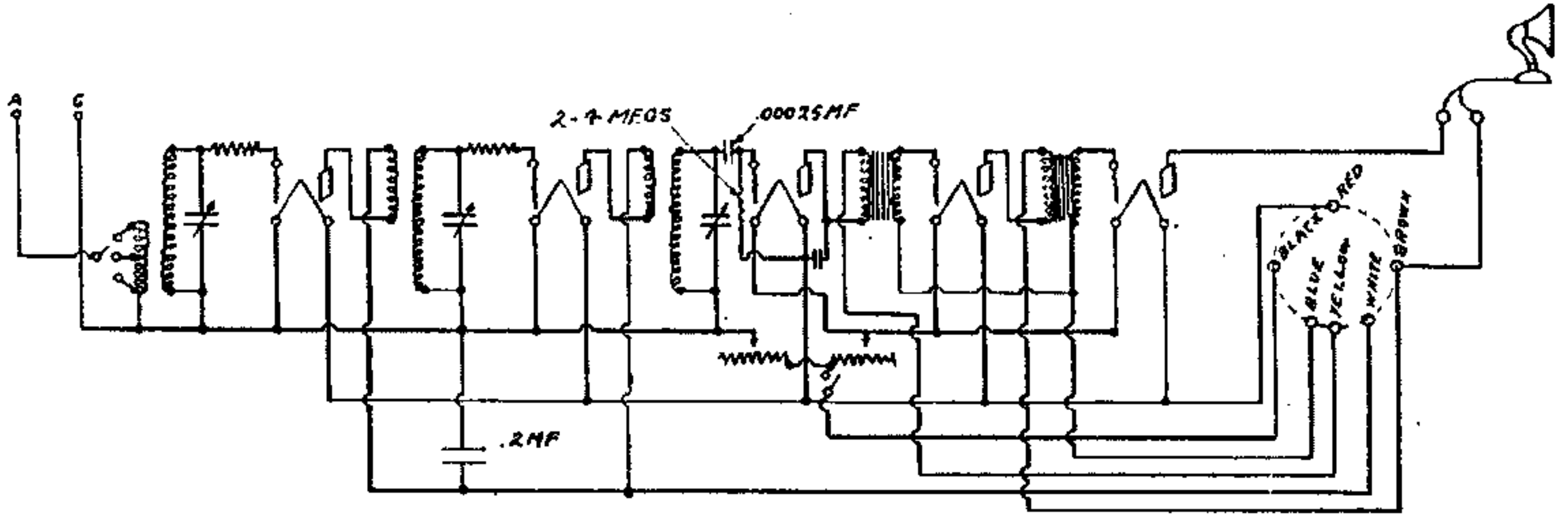
MODEL 20 COMPACT SET No. 7570. WIRING DIAGRAM
