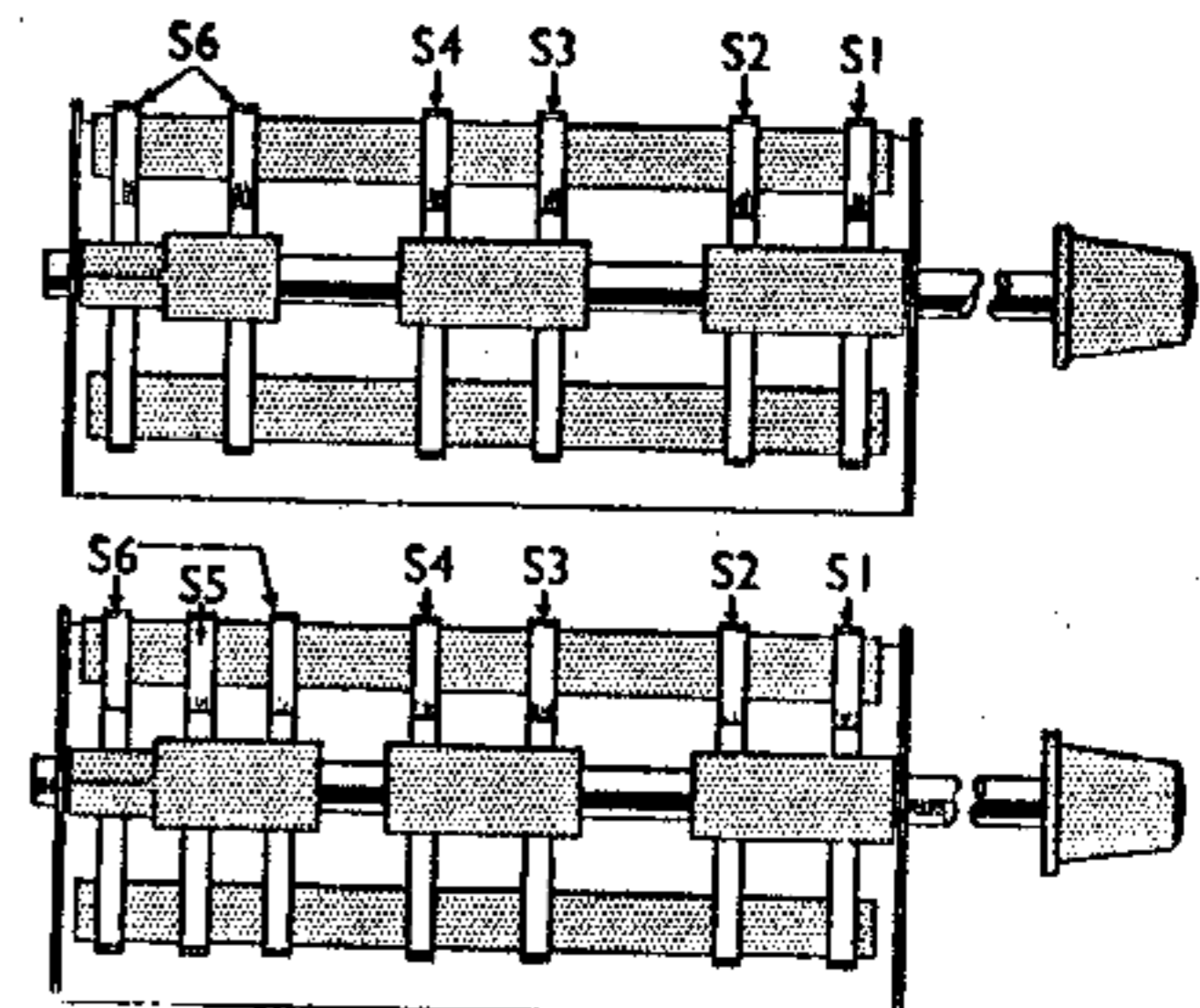
Sketches of the alternative waveband and scale lamp switch panels. That containing S5 occurs in chassis numbered above 3000. Earlier chassis only had the four waveband switches, S1-S4.
