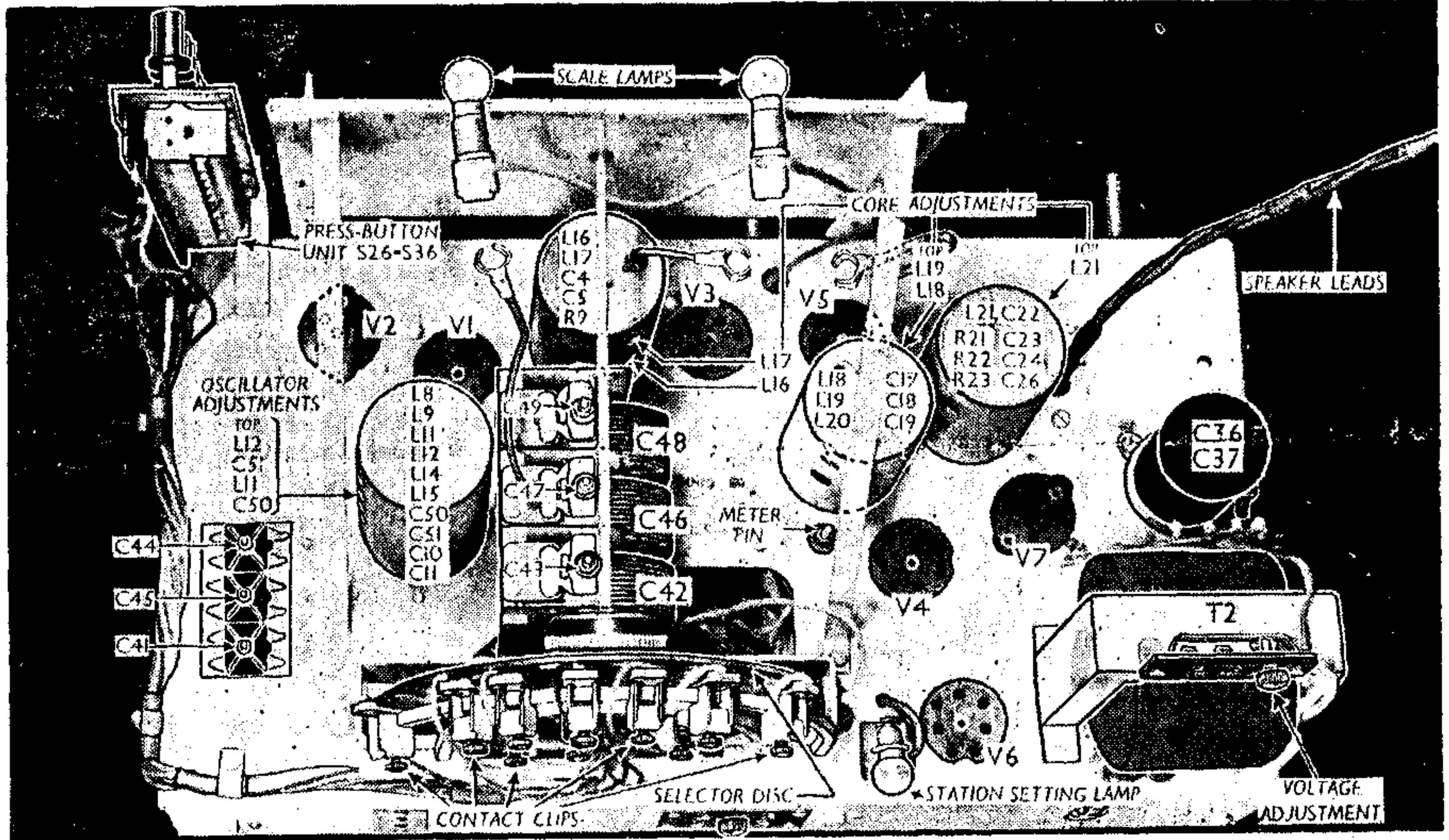
Right: [Plan] view of the chassis. All four screened coil units have core adjustments as indicated.
