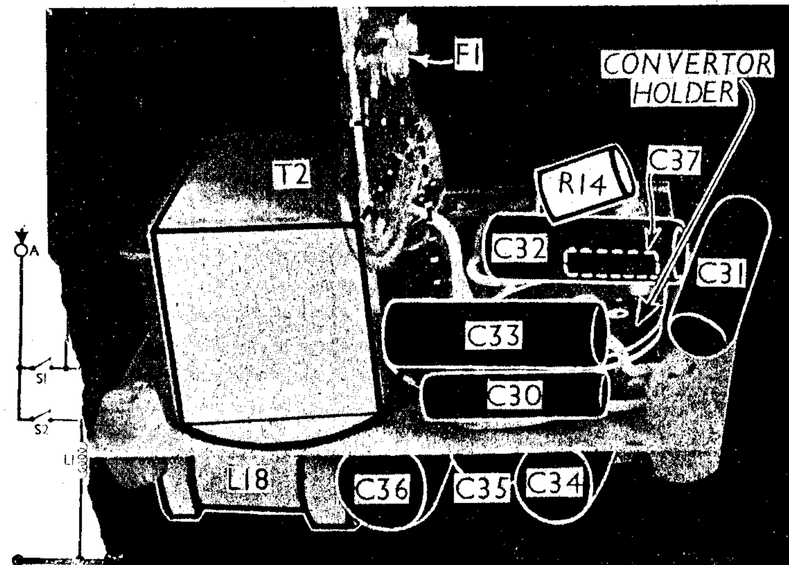
Three-quarter plan view of the converter unit assembly, showing the components above and below the chassis deck. The H.T. + lead and L.T. + lead from the receiver go to two tags, one either side of the fuse F1. The vibrator unit plugs into the holder indicated.
