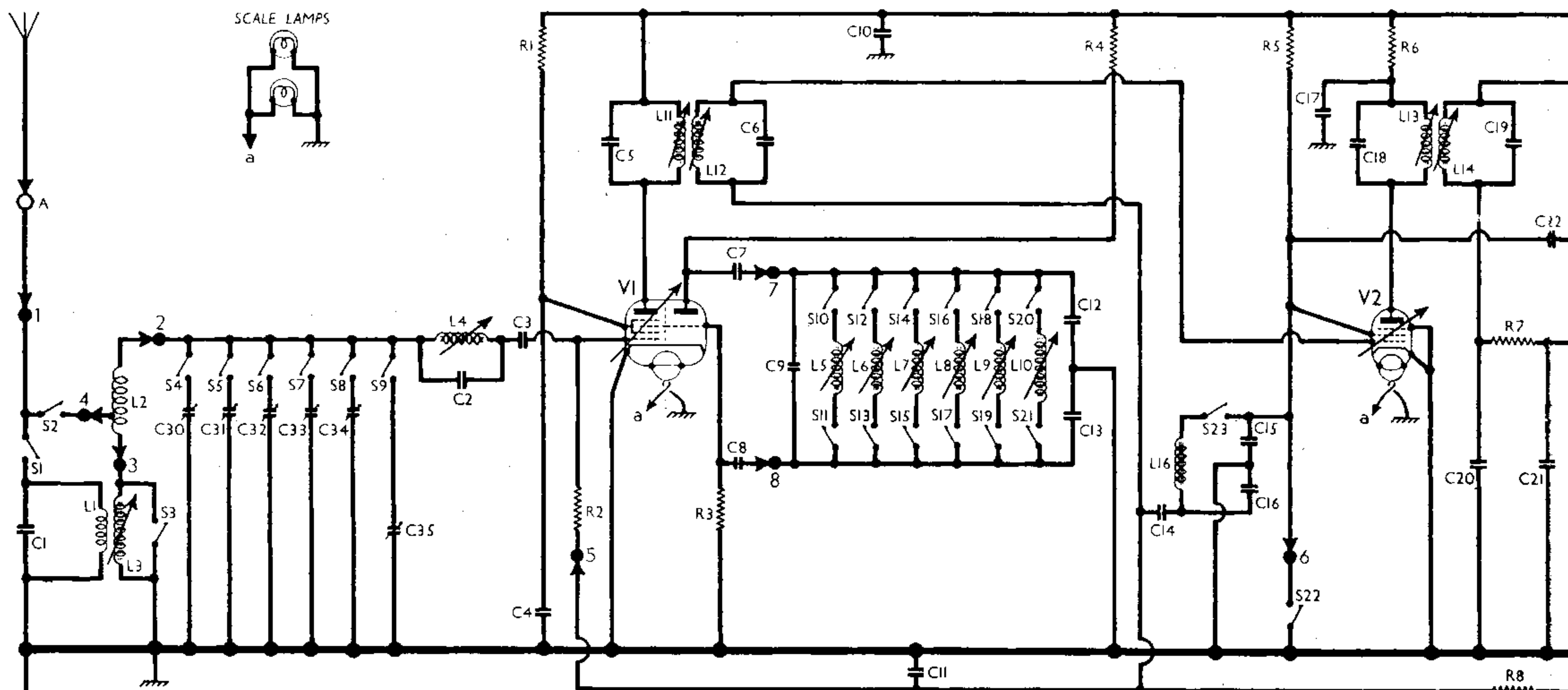
Circuit diagram of the Ekco A33 receiver. Although a frame aerial is used, provision is made for the connection of an external aerial via socket A. The numbered points in the diagram indicate the eight connections between the tuning assembly and the chassis, which are explained in detail under "Dismantling the Set." The radio muting switch S22 closes between settings of the station selector control, and S23 is closed when the "Tone Alarm" facility is required. Relay winding L17 has a dual function, since it closes its associated contacts S26 , in the mains circuit, and also acts as an H.T. smoothing choke.
