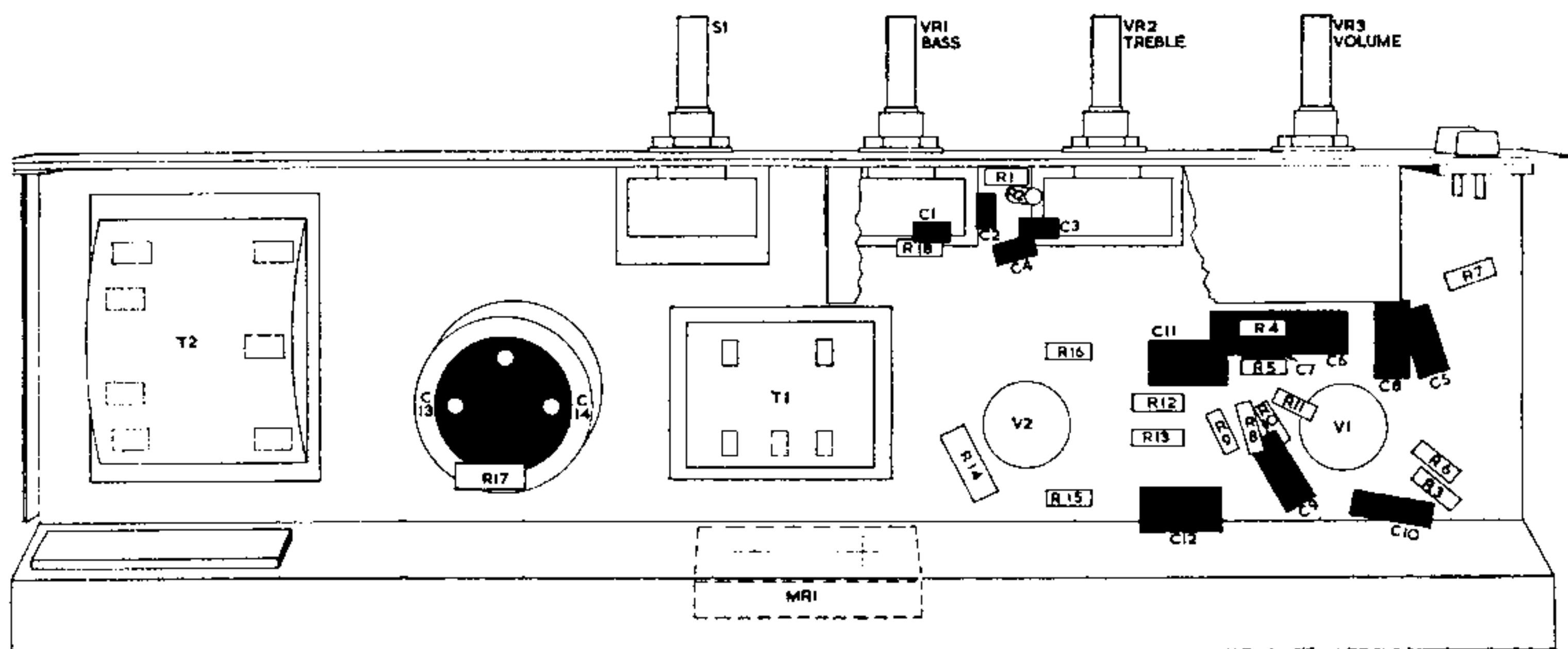
LAY-OUT DIAGRAM—DECCA MODEL RP205
