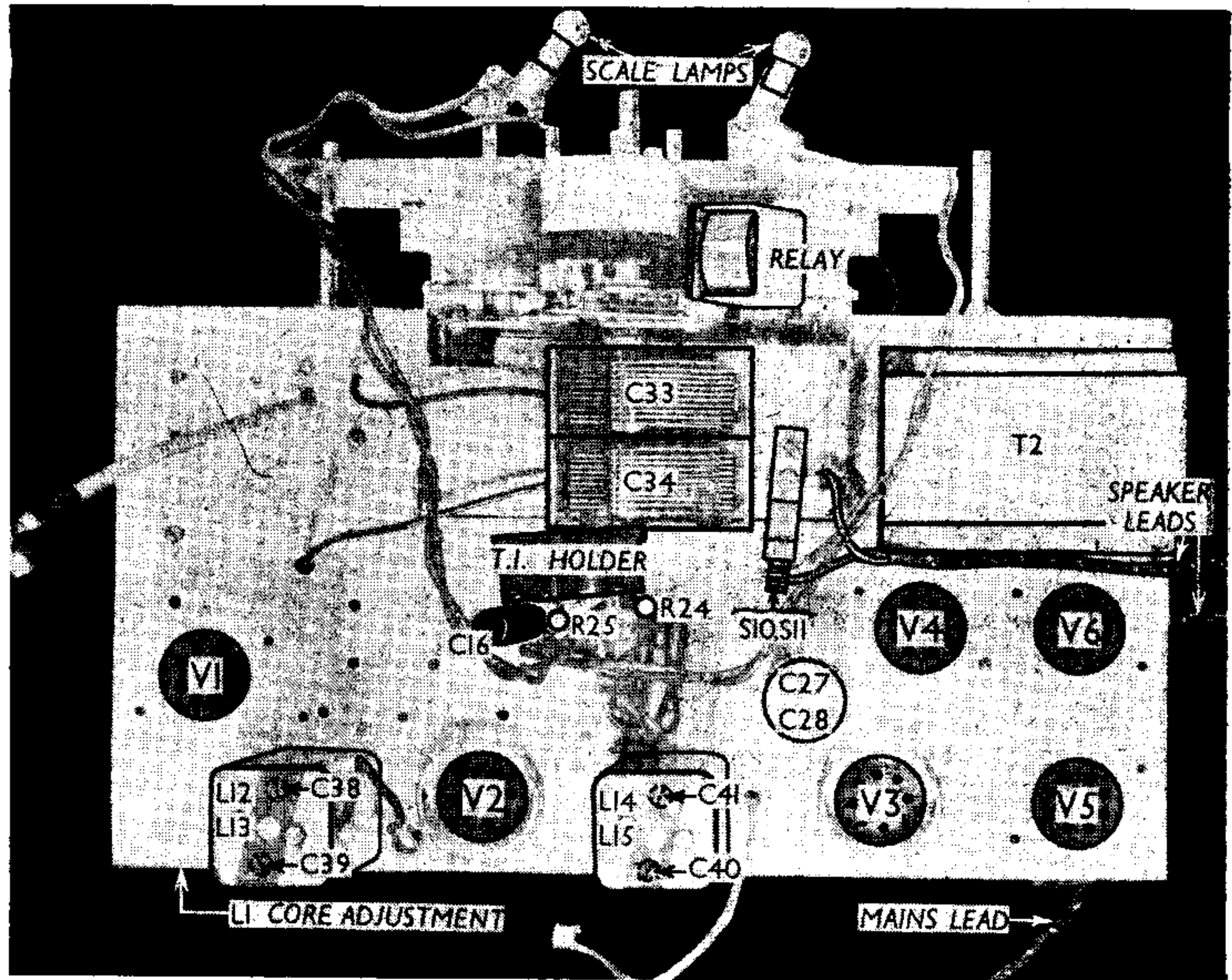
Plan view of the chassis. S10, S11 are leaf switches for muting the speaker and operating the relay when a button is pressed. The relay is also shown.
