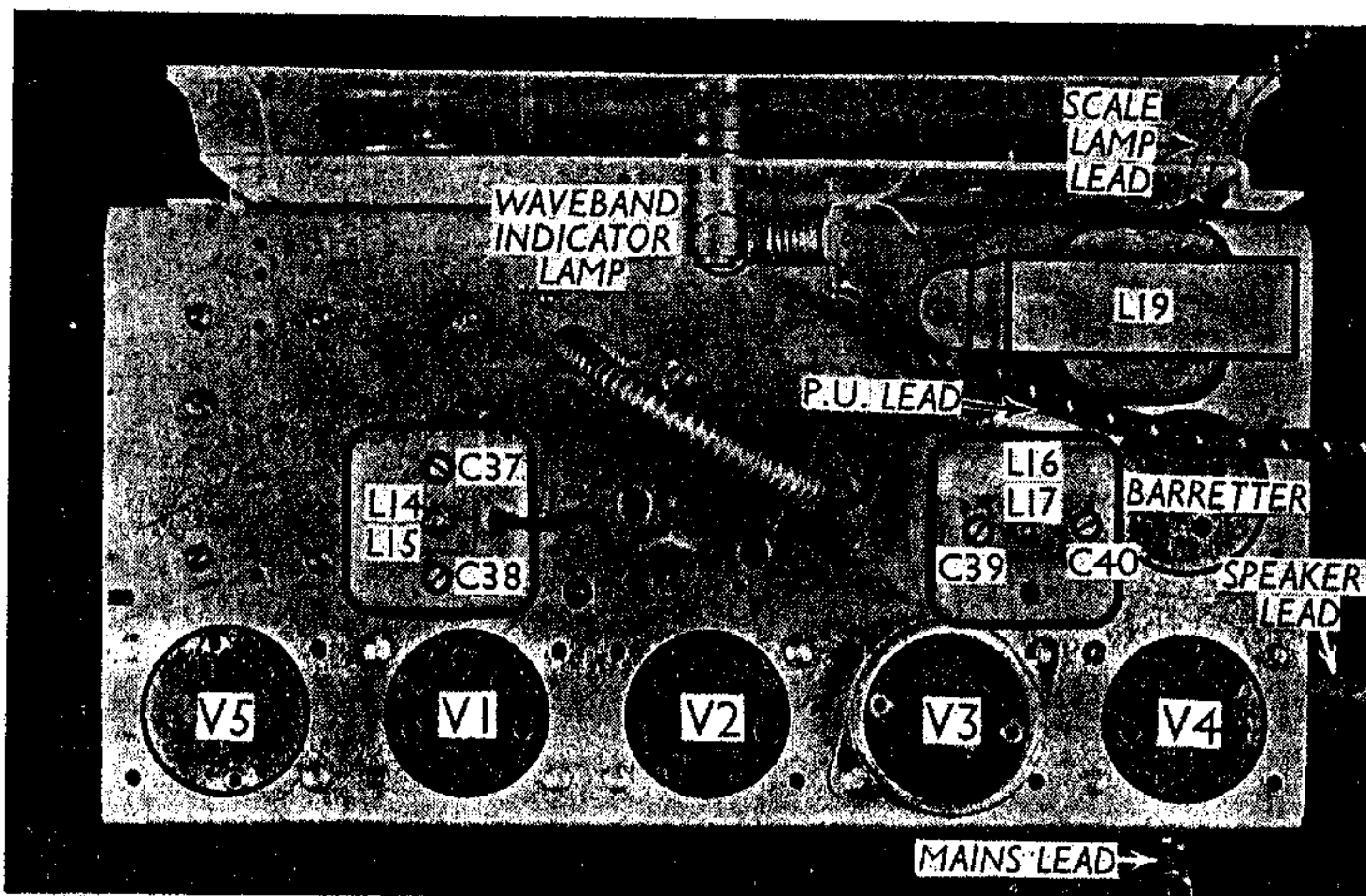
Plan view of the chassis. The two I.F. transformers and their trimmers are shown, but all the other tuning coils are beneath the chassis.
