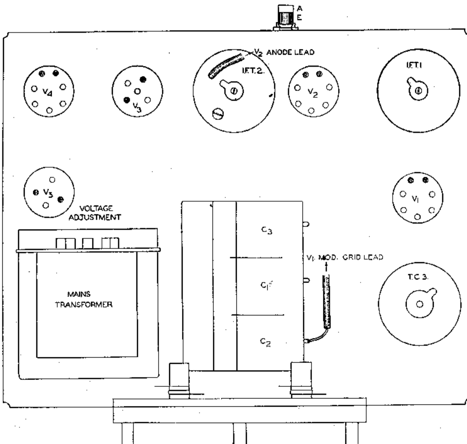
PLAN VIEW OF TOP OF CHASSIS
