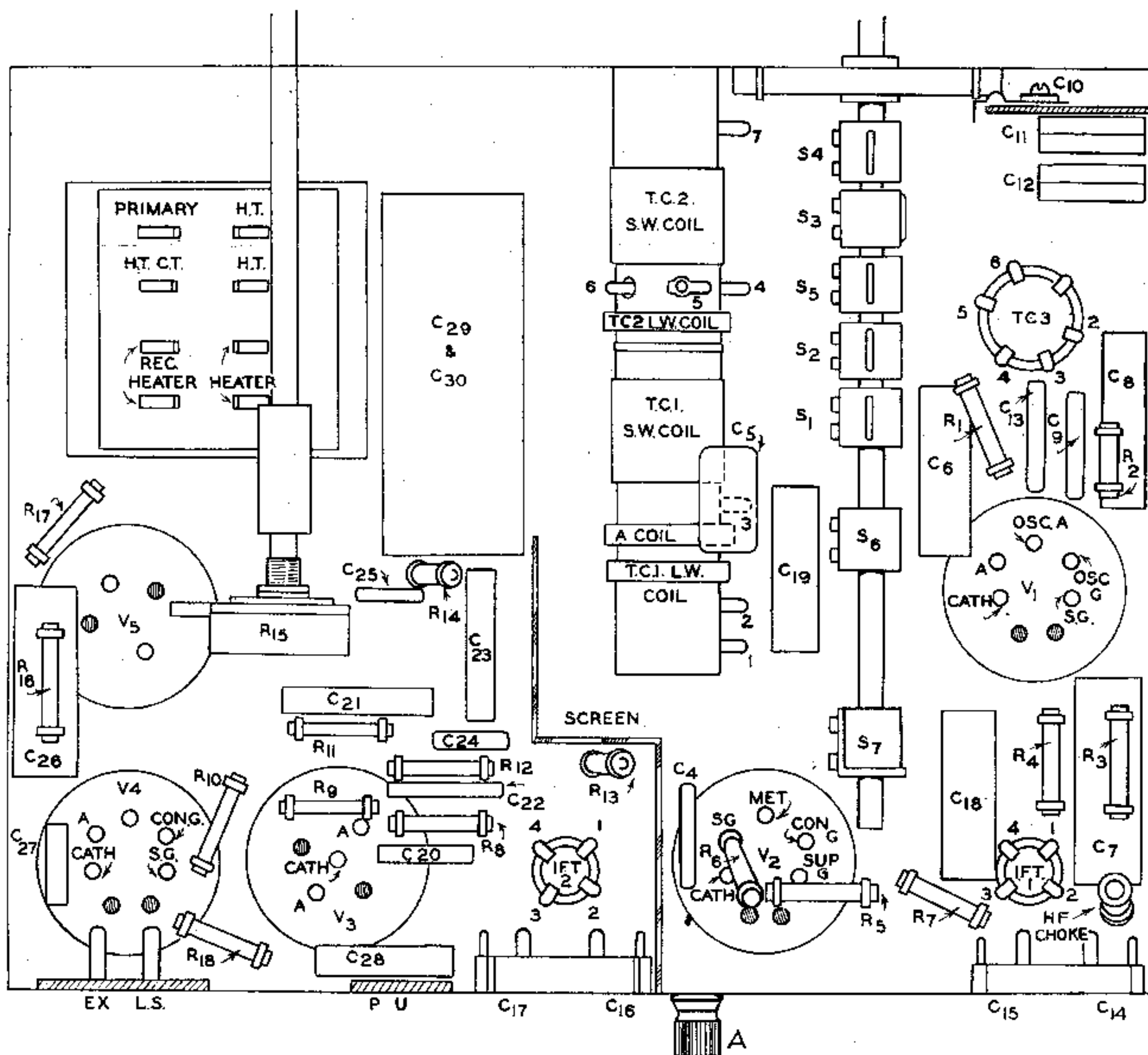
UNDERSIDE VIEW OF CHASSIS
