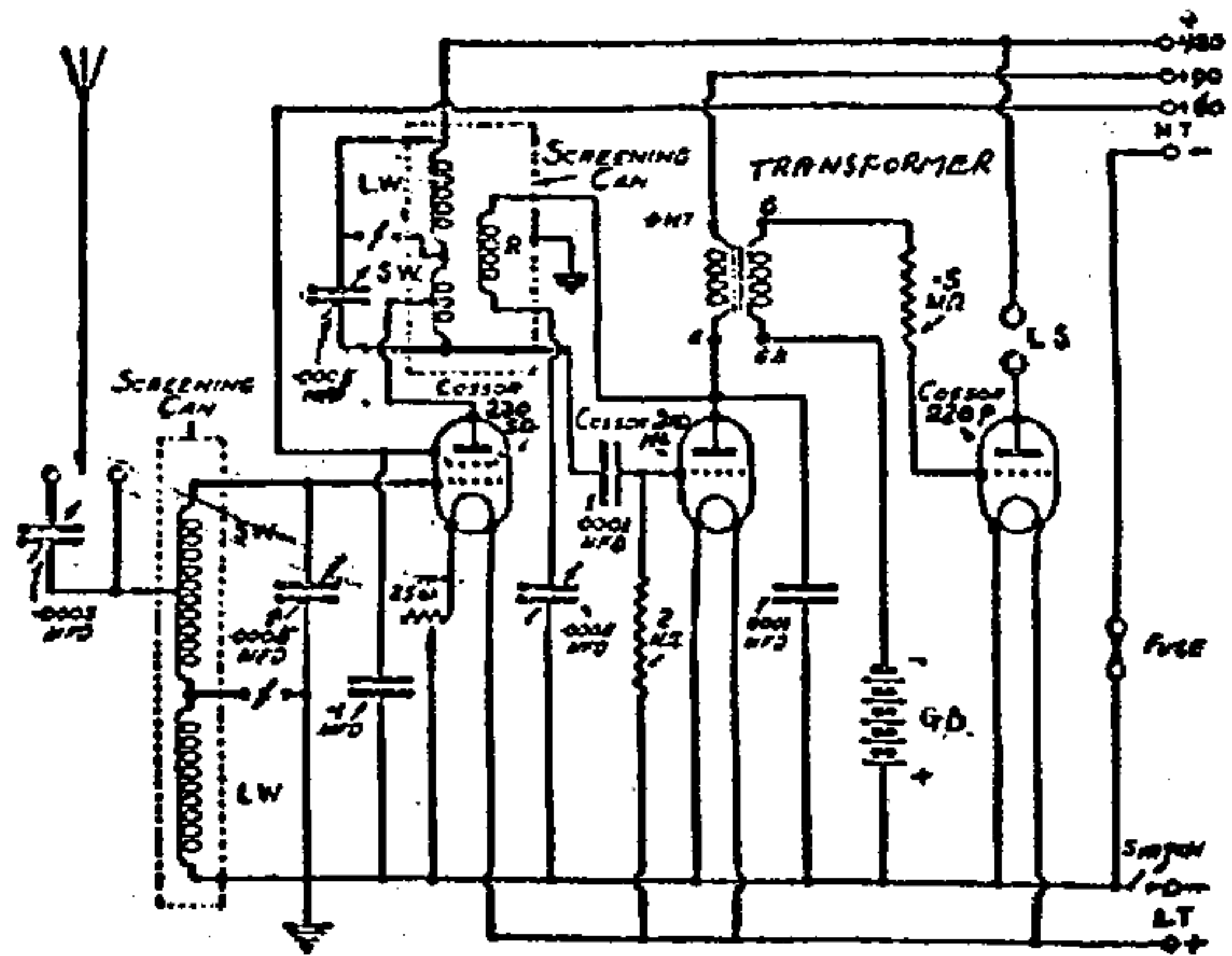
The New Cossor Empire Melody Maker (Model 234)
