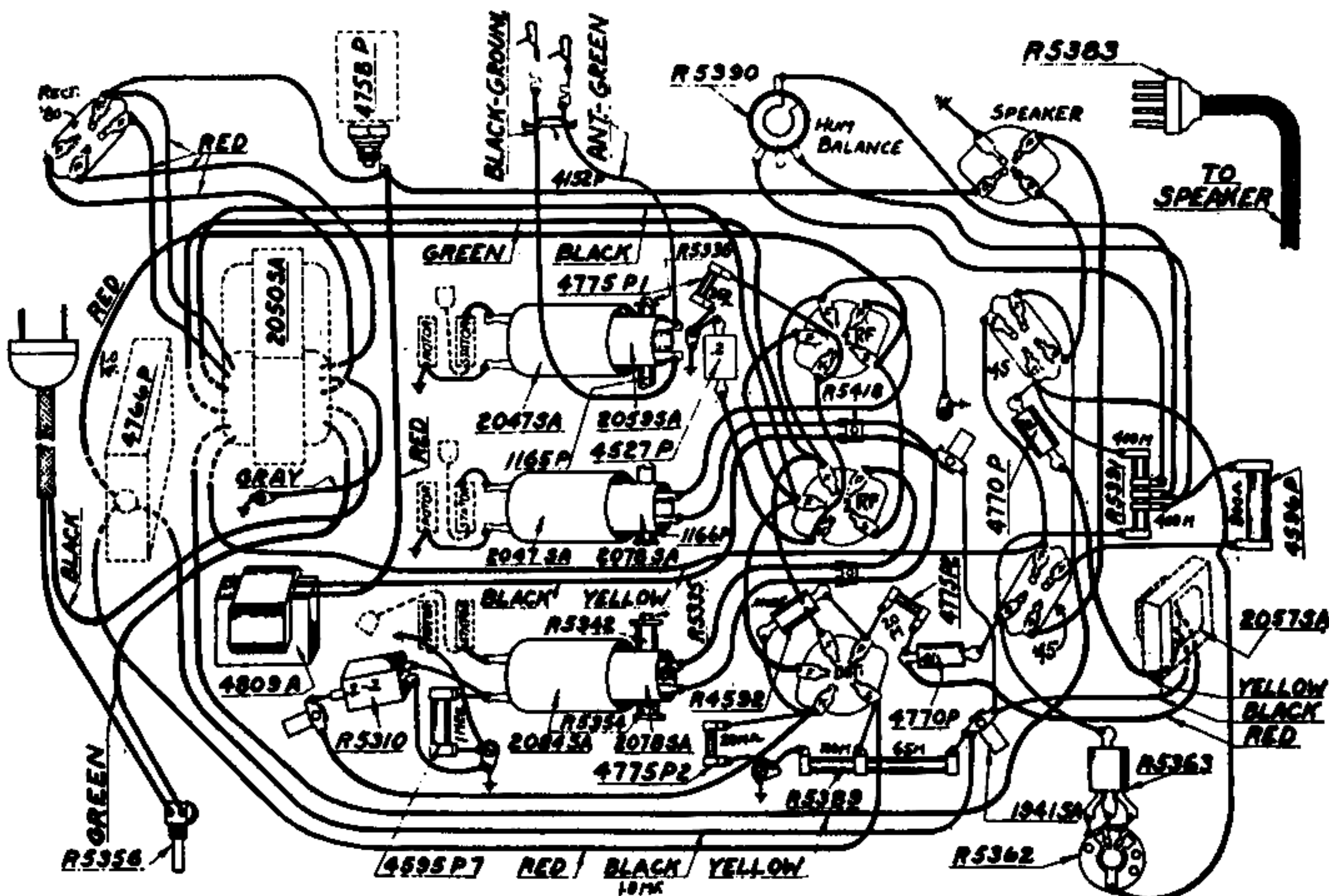
CHASSIS WIRING
