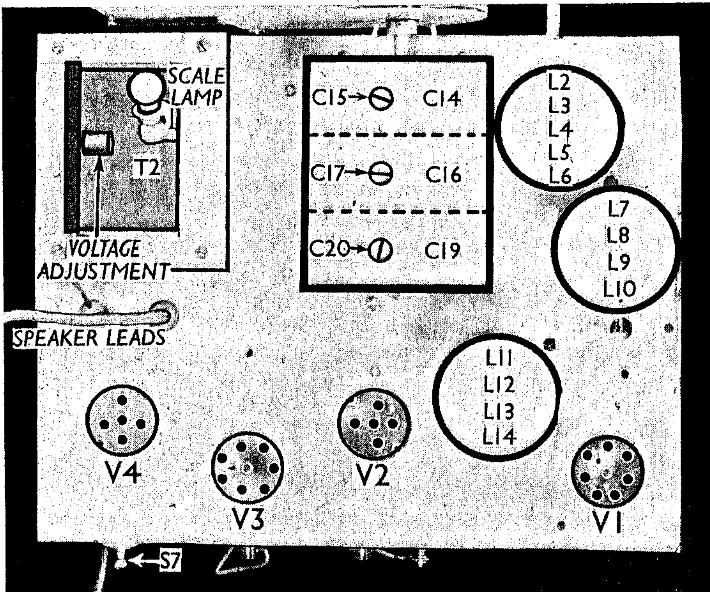
Plan view of the chassis. S7 at the rear is the tone control switch.
