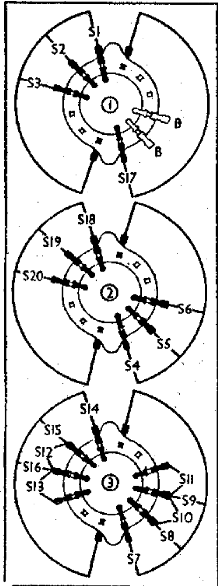
Diagrams of the switch units as seen looking from the rear of the underside of the chassis. The radiogram model has an extra unit, as explained under "General Notes."
