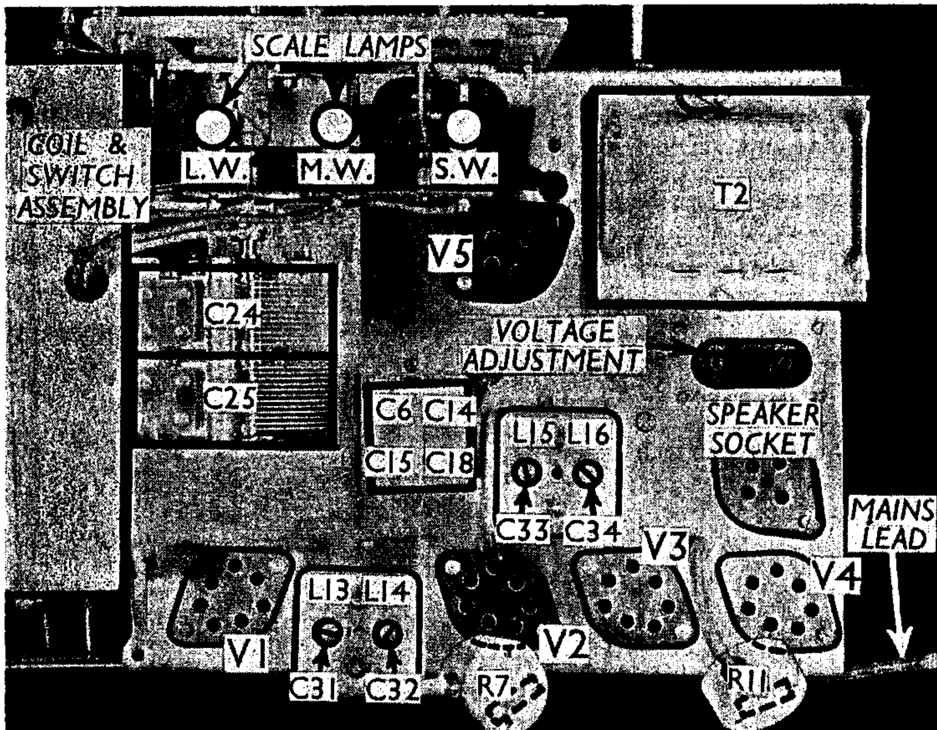
Plan chassis view. Note R7 and R11 inside the valve top cap connectors.
