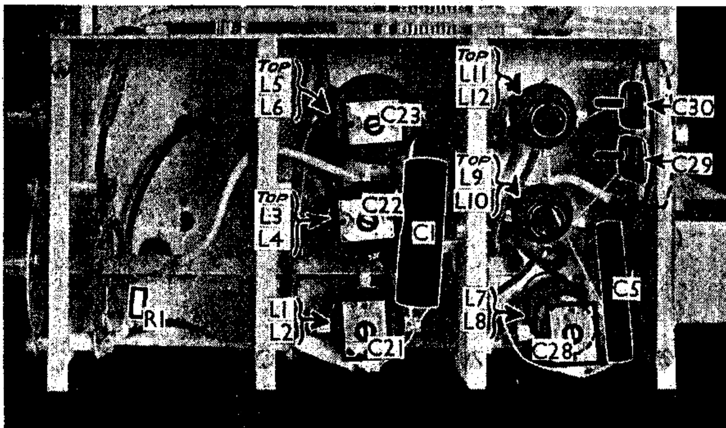
Side-chassis view, with the cover plate removed. Each coil unit contains two coils, and four of them have trimmers at their ends.
