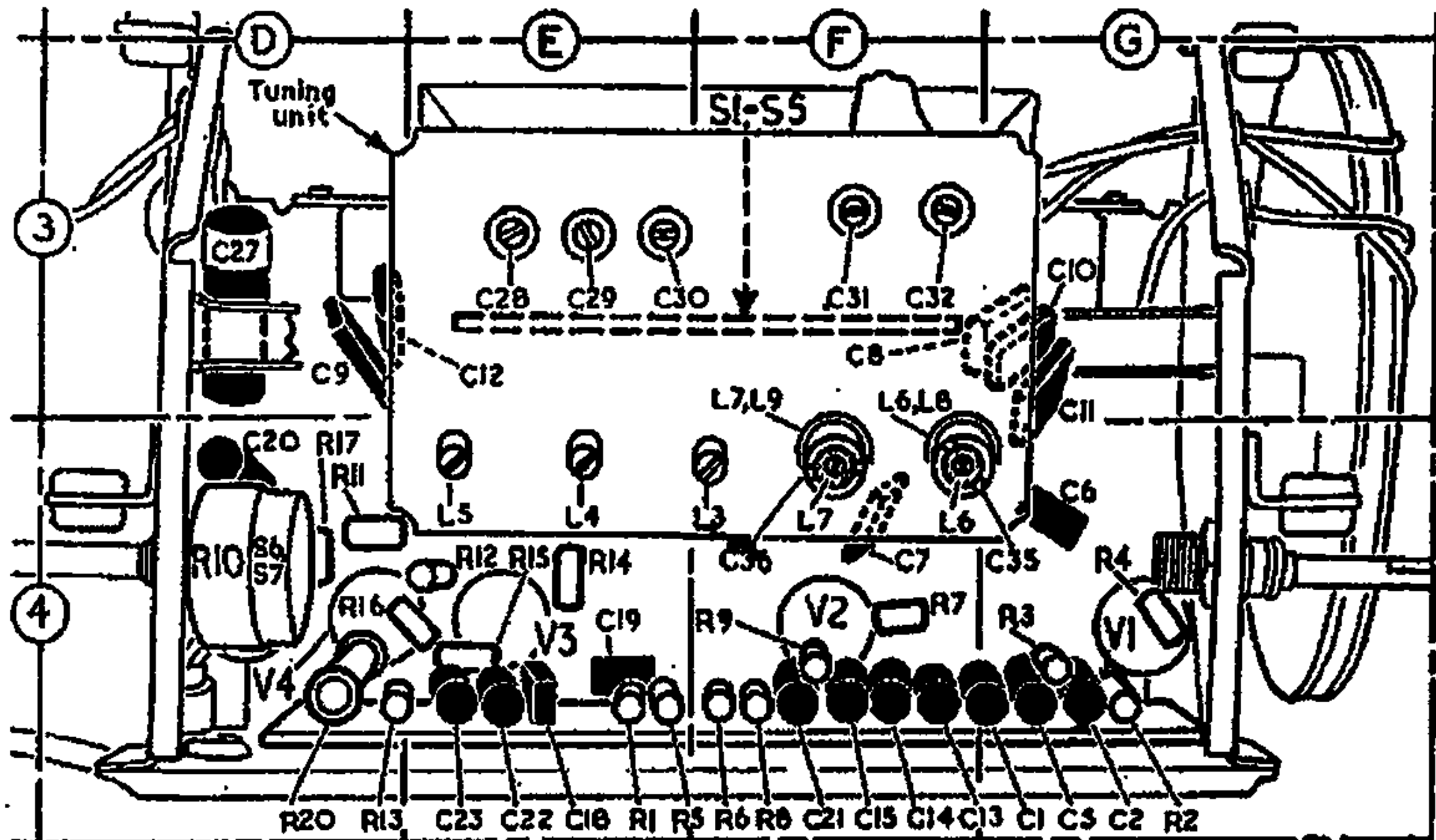
Underside drawing of the chassis, with the tuning unit in position. All the R.F. and oscillator alignment adjustments are indicated here. A separate drawing of the tuning unit after removal appears at the foot of this page.
