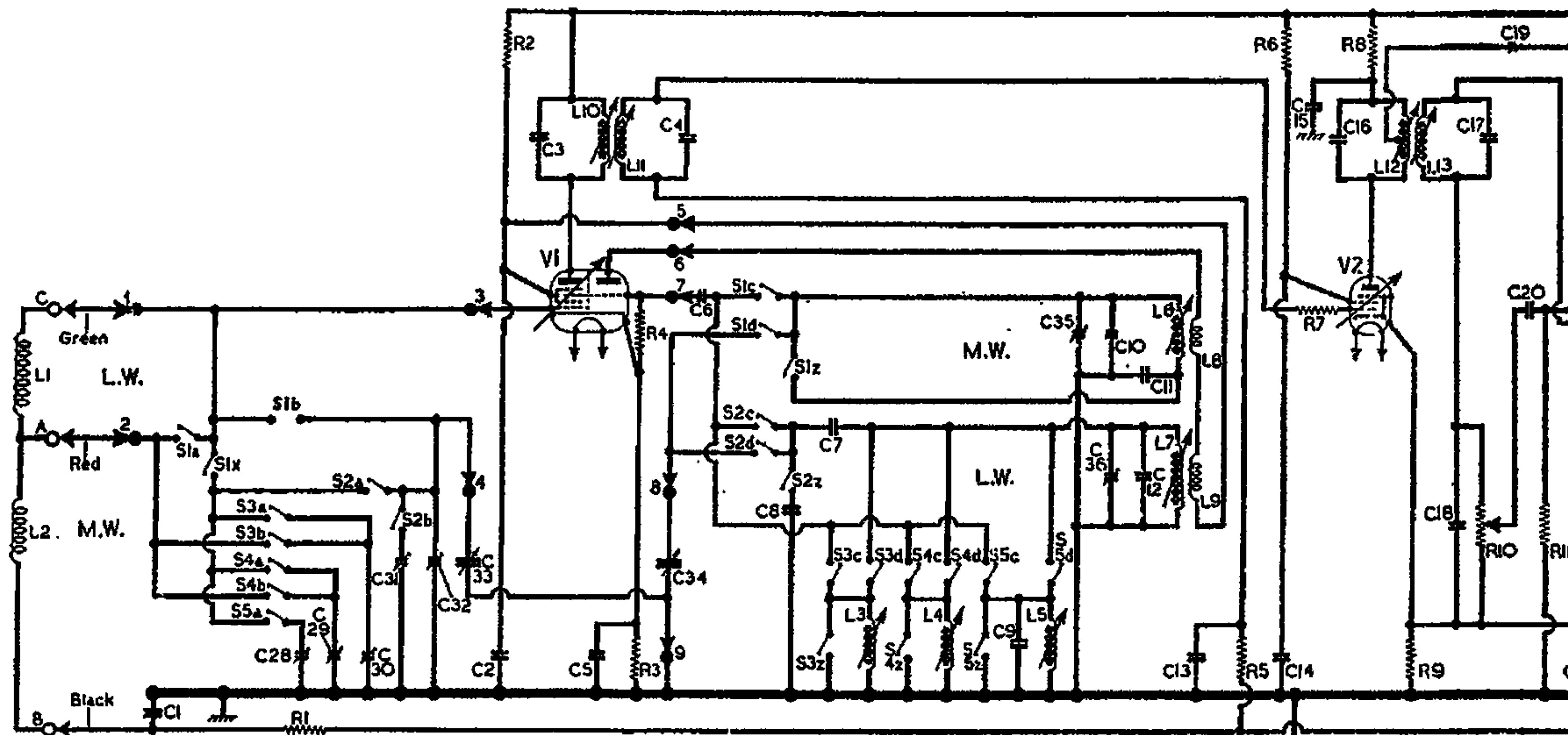
Circuit diagram of the Bush DAC10 A.C./D.C. superhet. No provision is made for the connection of an external aerial. The frame aerial connections are lettered A, B and C, and the connections between the chassis and the tuning unit are numbered 1 to 9. Note that M.W. is the lower coil in the aerial circuit, and the upper coil in the oscillator.
