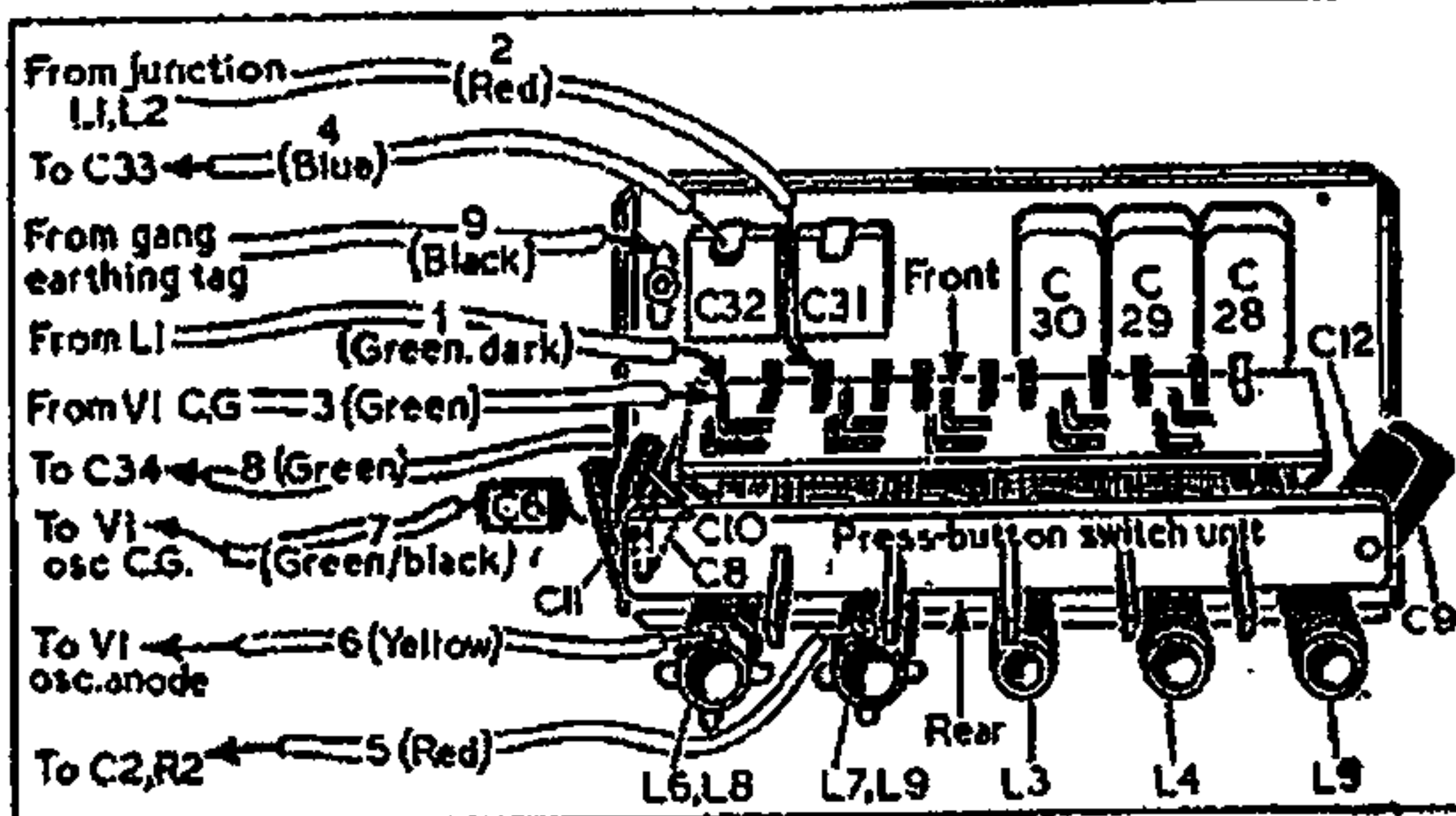
Sketch of the tuning unit after removal from the chassis. All the connecting leads (numbered 1 to 9) between the unit and the chassis are identified here. An arrow-head indicates the end of the lead that is unsoldered in our dismantling instructions.
