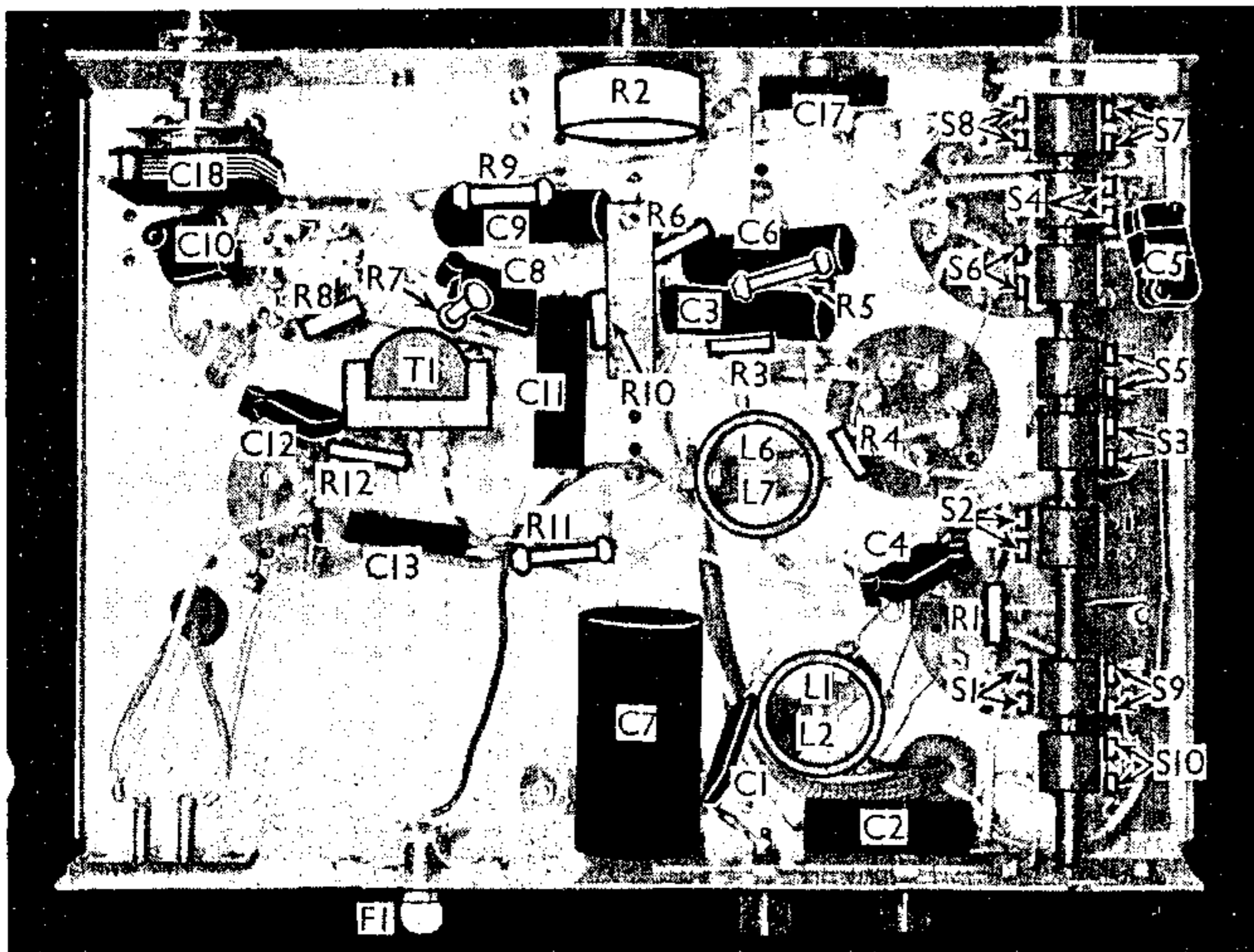
Under-chassis view. L1, L2 and L6, L7 are the S.W. coils. F1 is a fuse bulb. All the switches are included in the unit on the right.
