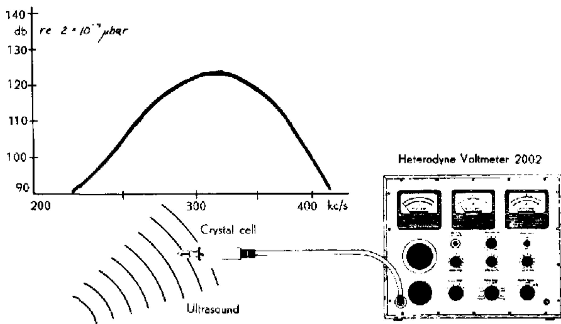
Fig. 17. Measurement and analysis of airborne ultrasound.
