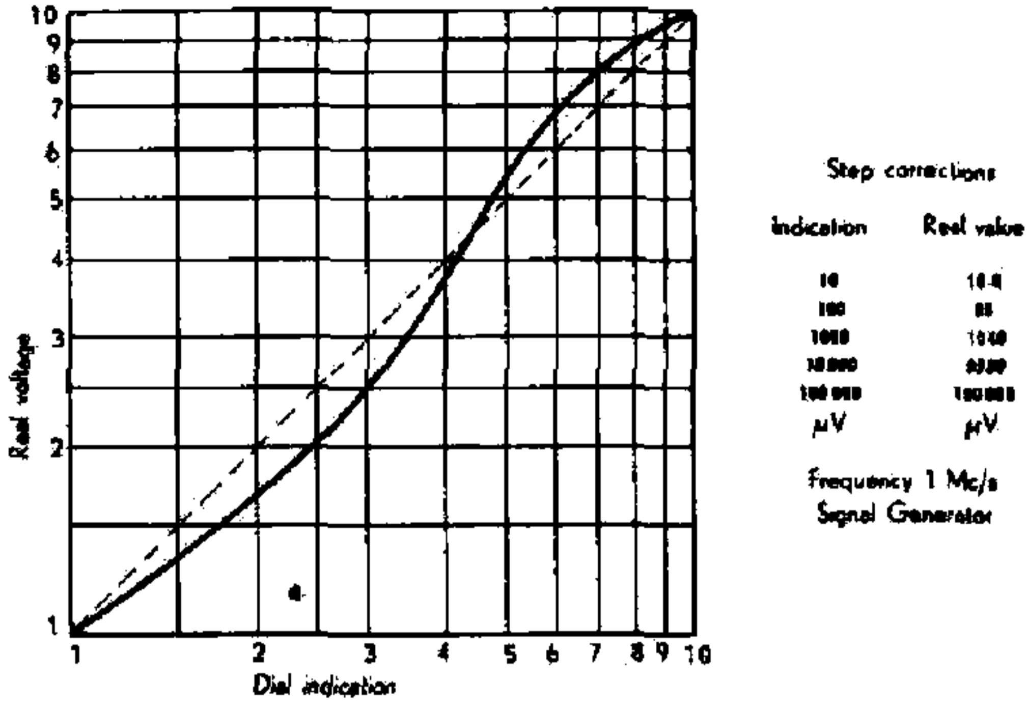
Fig. 6. Correction curve for a laboratory signal generator.
