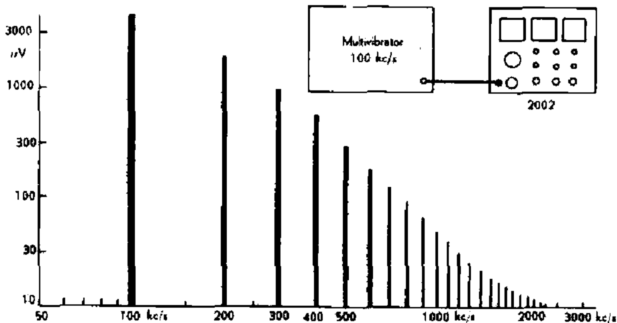
Fig. 8. Spectrum of harmonics from a multi-vibrator.
