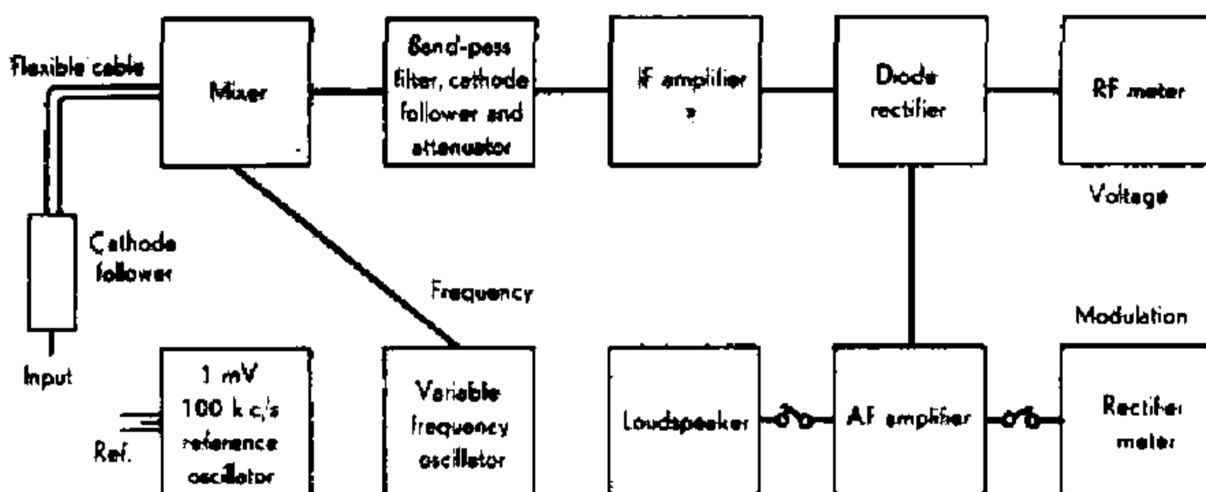
Fig. 2. Block diagram of the Heterodyne Voltmeter.
