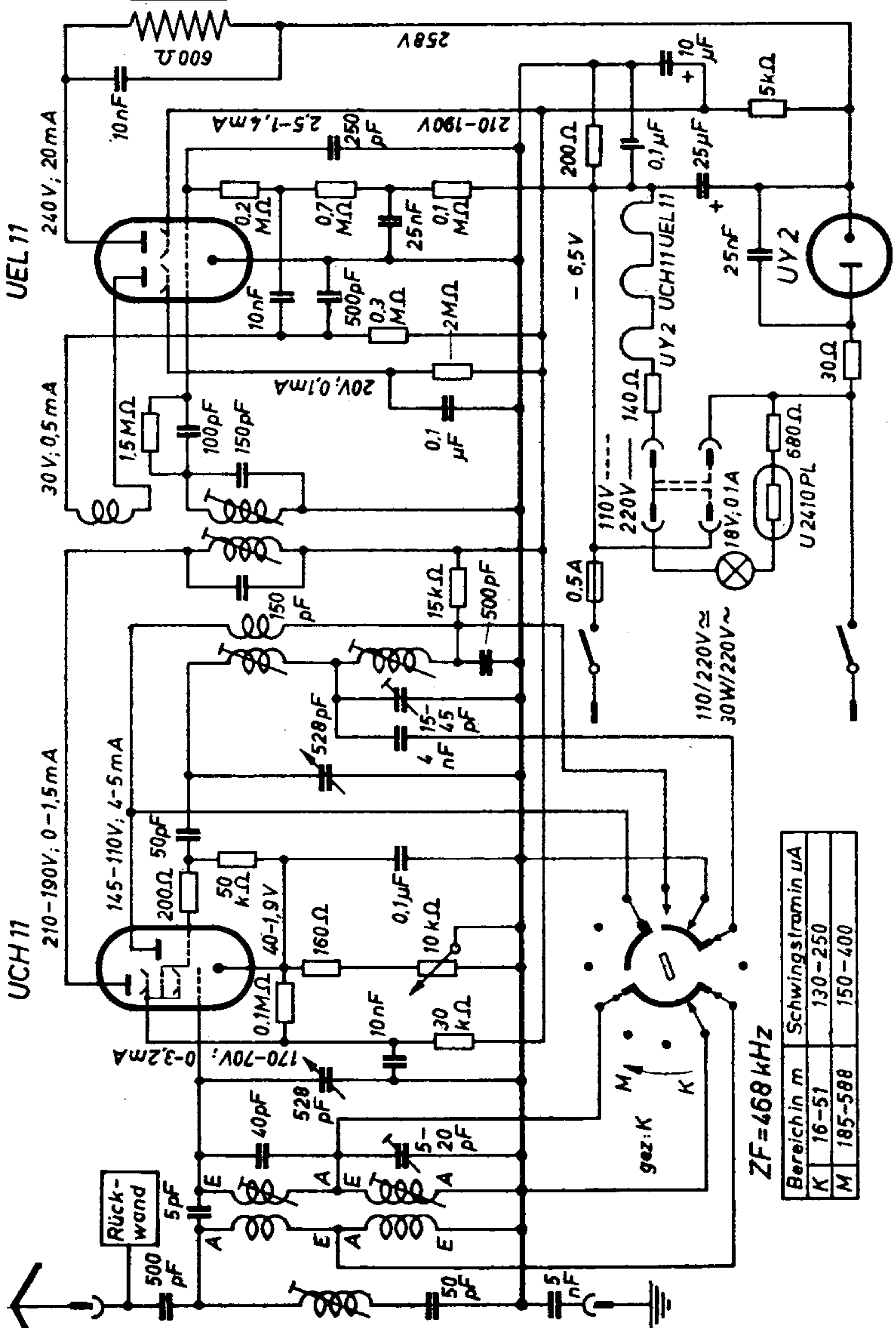
Brandt Favorit 3449 GWII/KM
