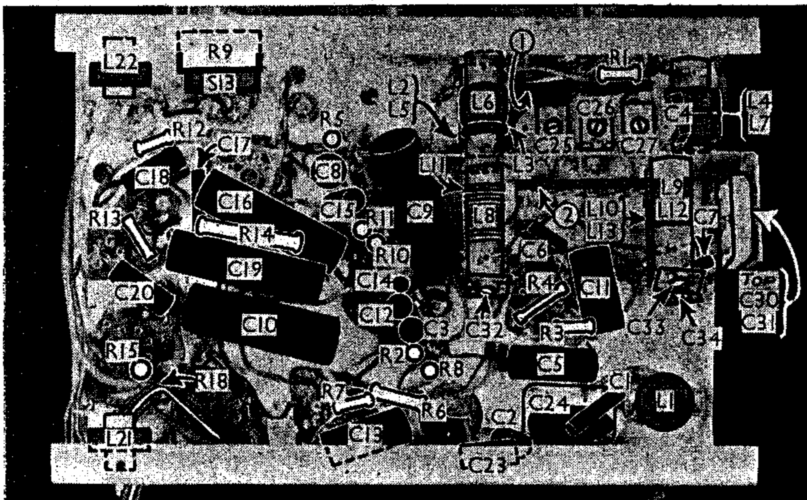
Under-chassis view. The two waveband switch units are indicated.
