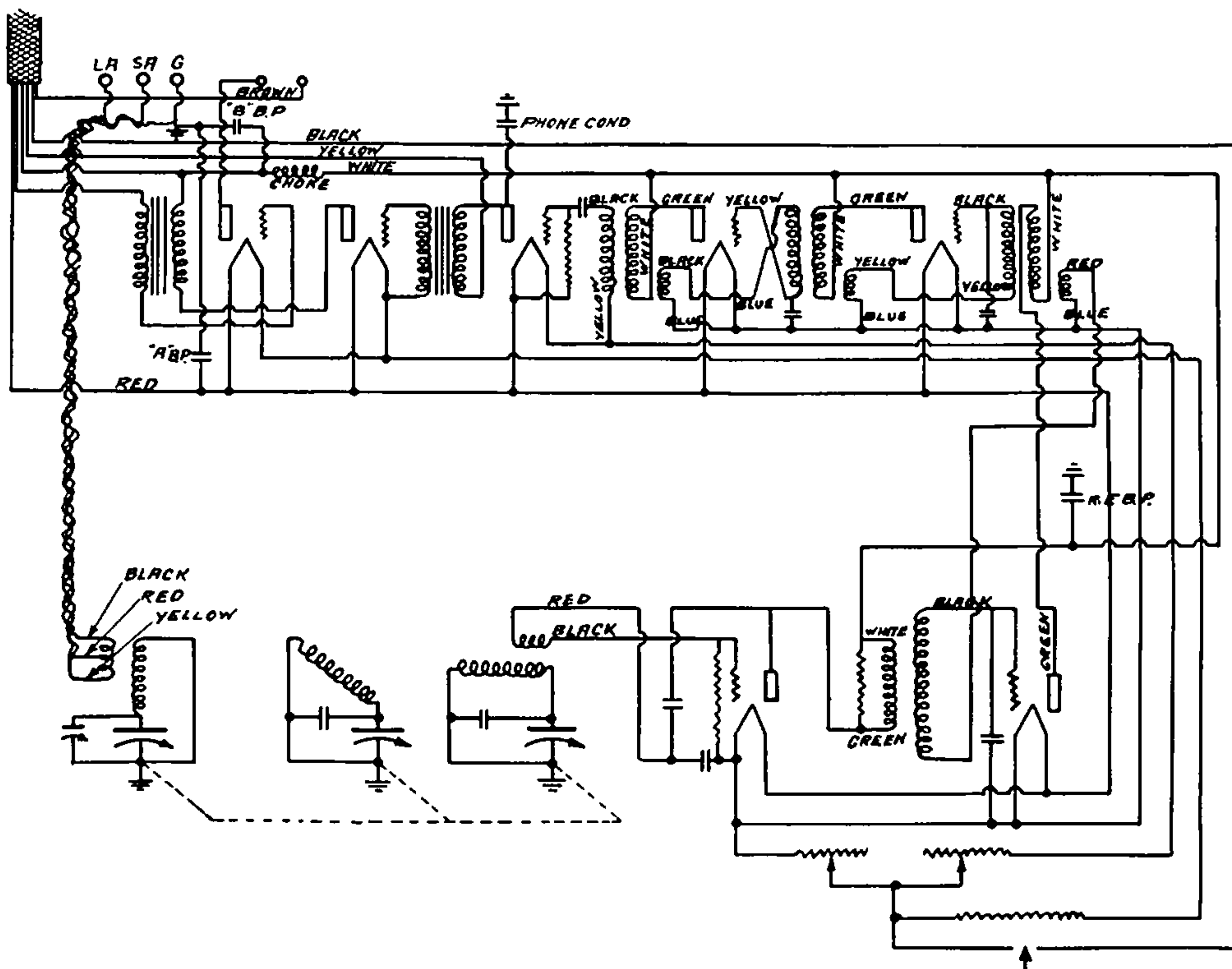
FIG. 117. WIRING DIAGRAM OF MODEL 50.
