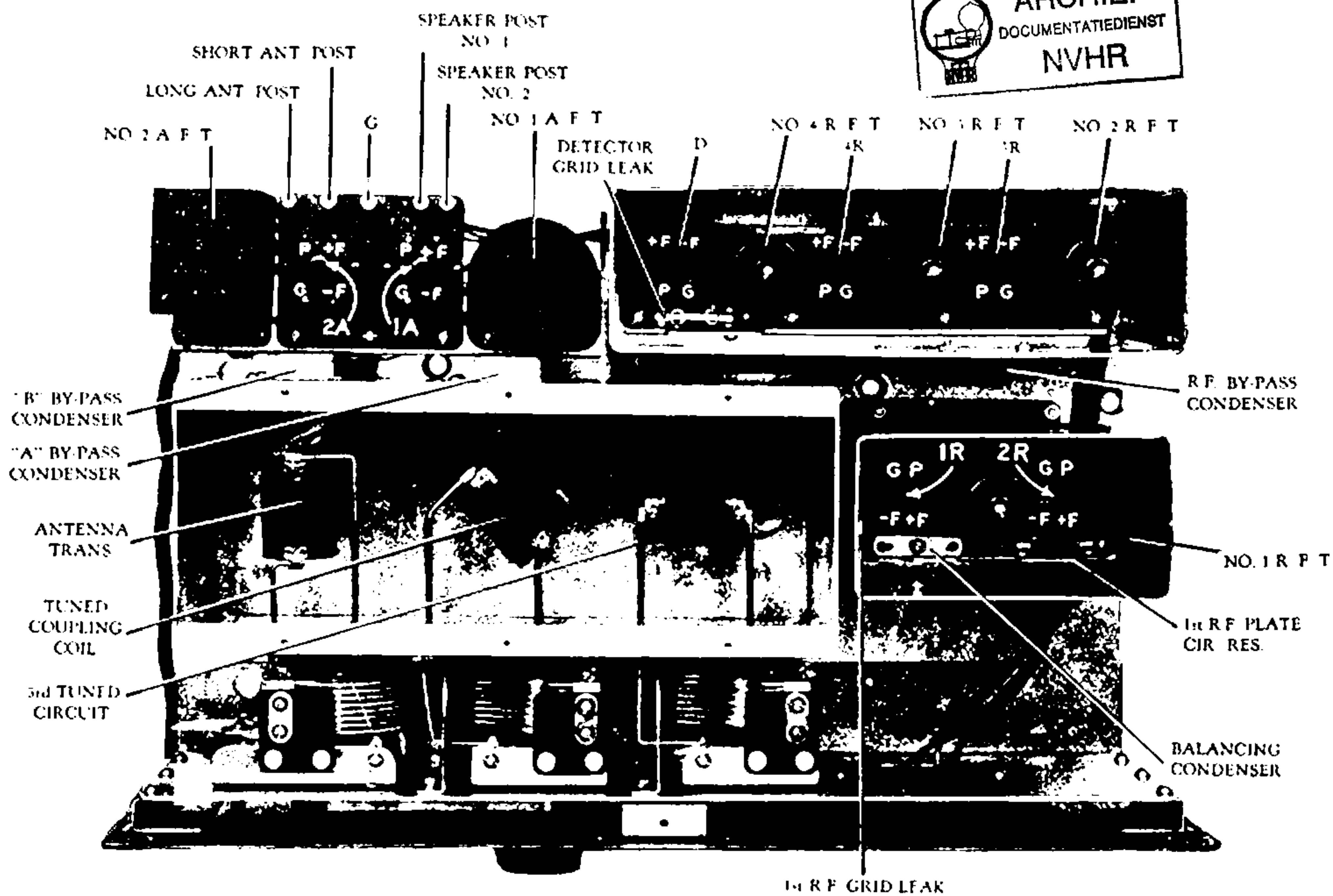
FIG. 116. TOP VIEW OF MODEL 50.
