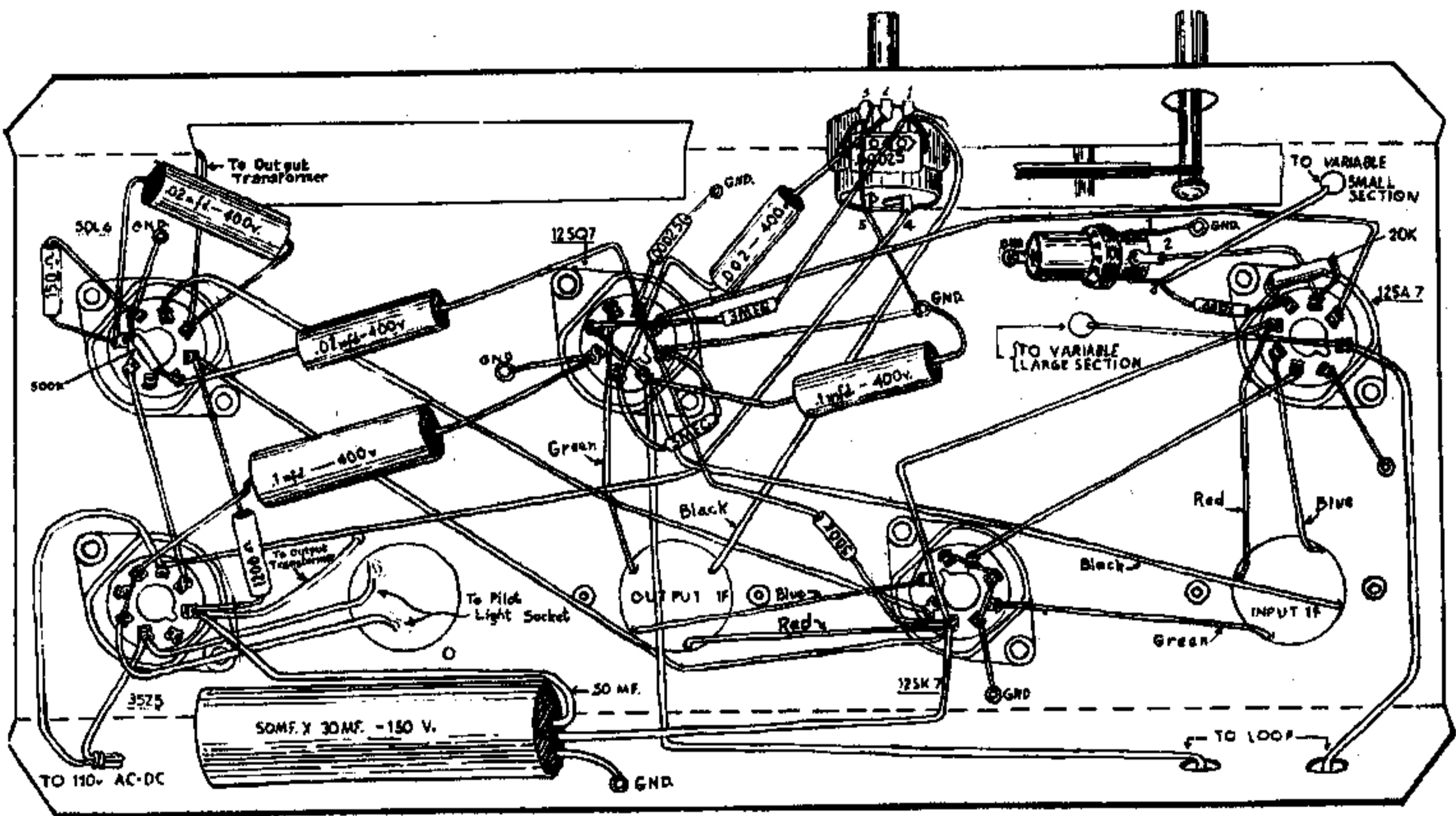
PICTORIAL DIAGRAM OF MODEL S-5C
