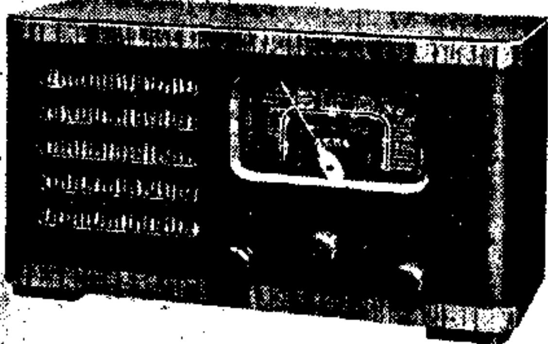
The Alba "Clipper" midget superhet receiver.
