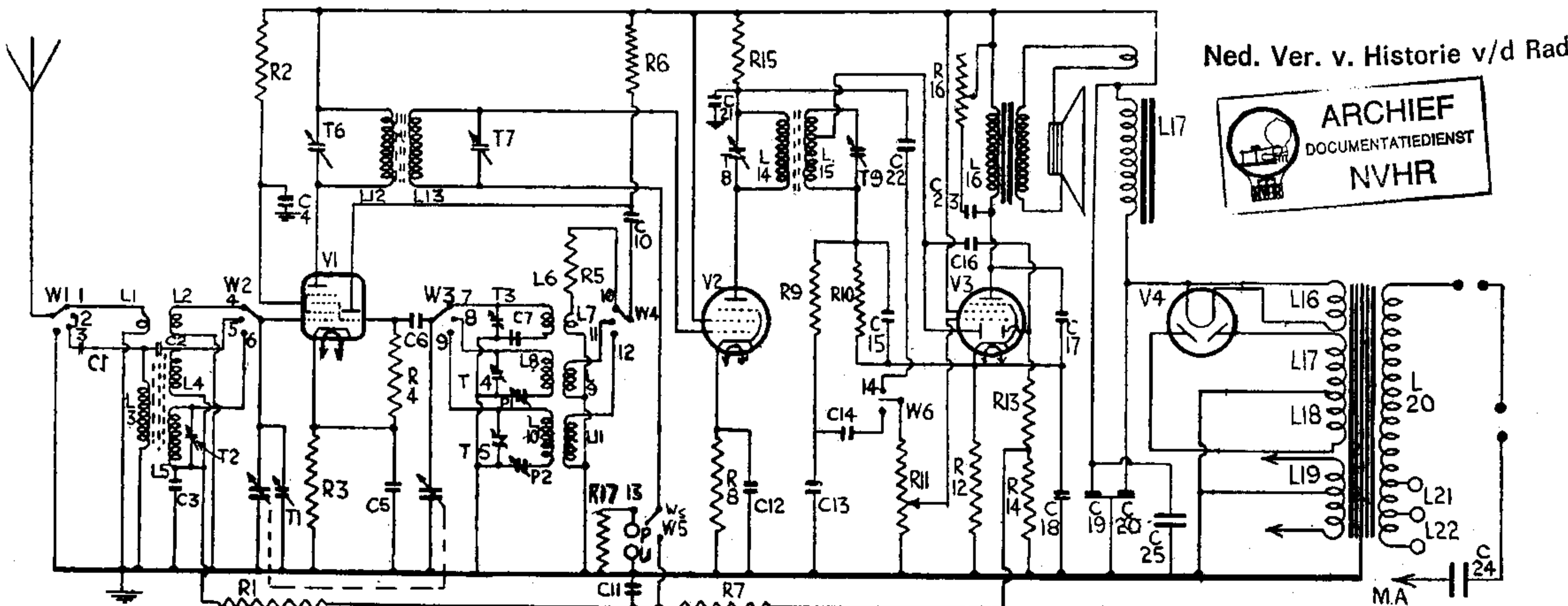
A conventional "short" superhet circuit is found in the model 90. The automatic tuning, being solely mechanical, does not involve any special circuit features.
