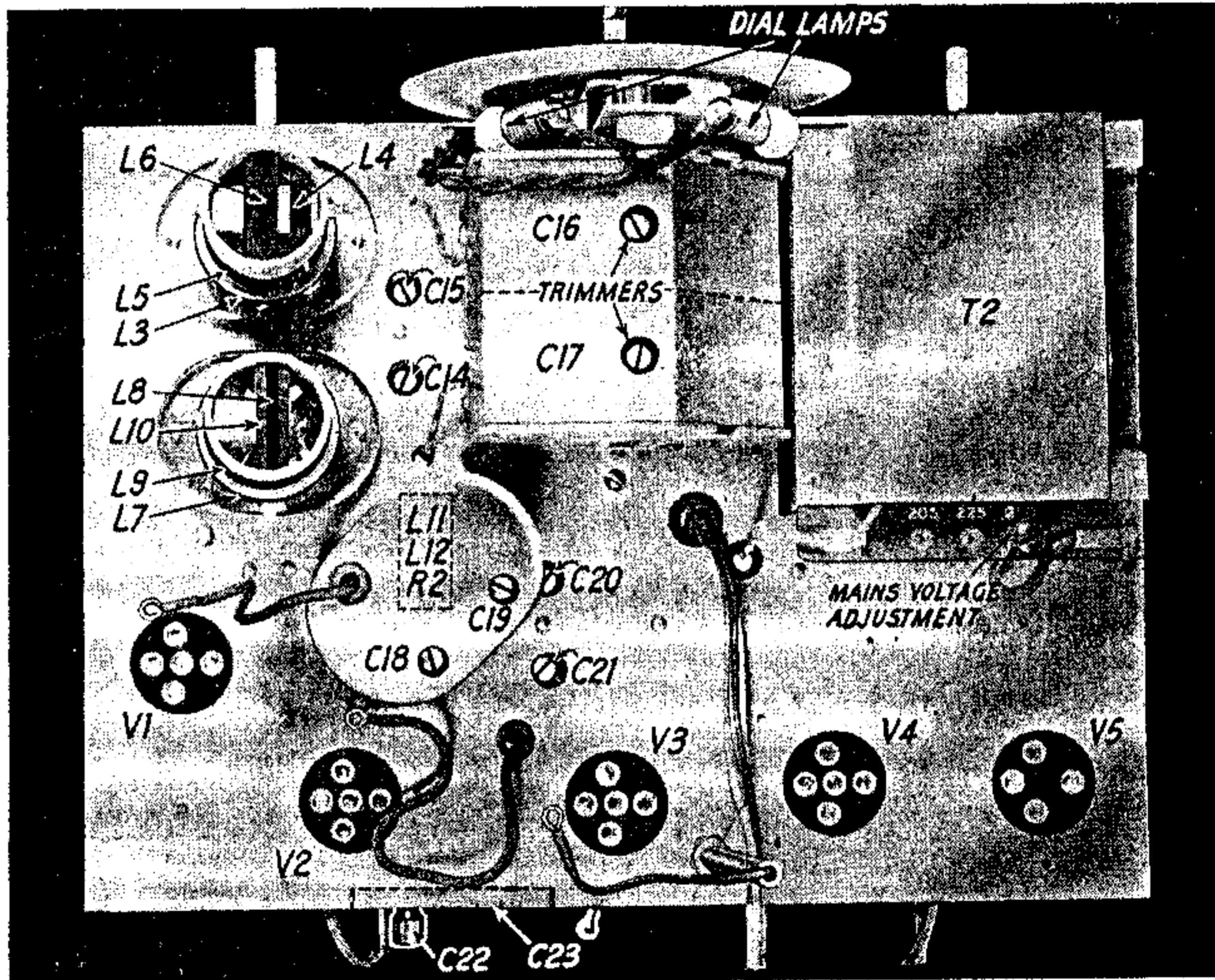
Fig. 3.—Plan view of the chassis. The valves and two of the coil screens have been removed. The third screen encloses L11, L12 and R2, also the trimmers C18 and C19. Note also the trimmers of C16 and C17, which are not separately numbered.
