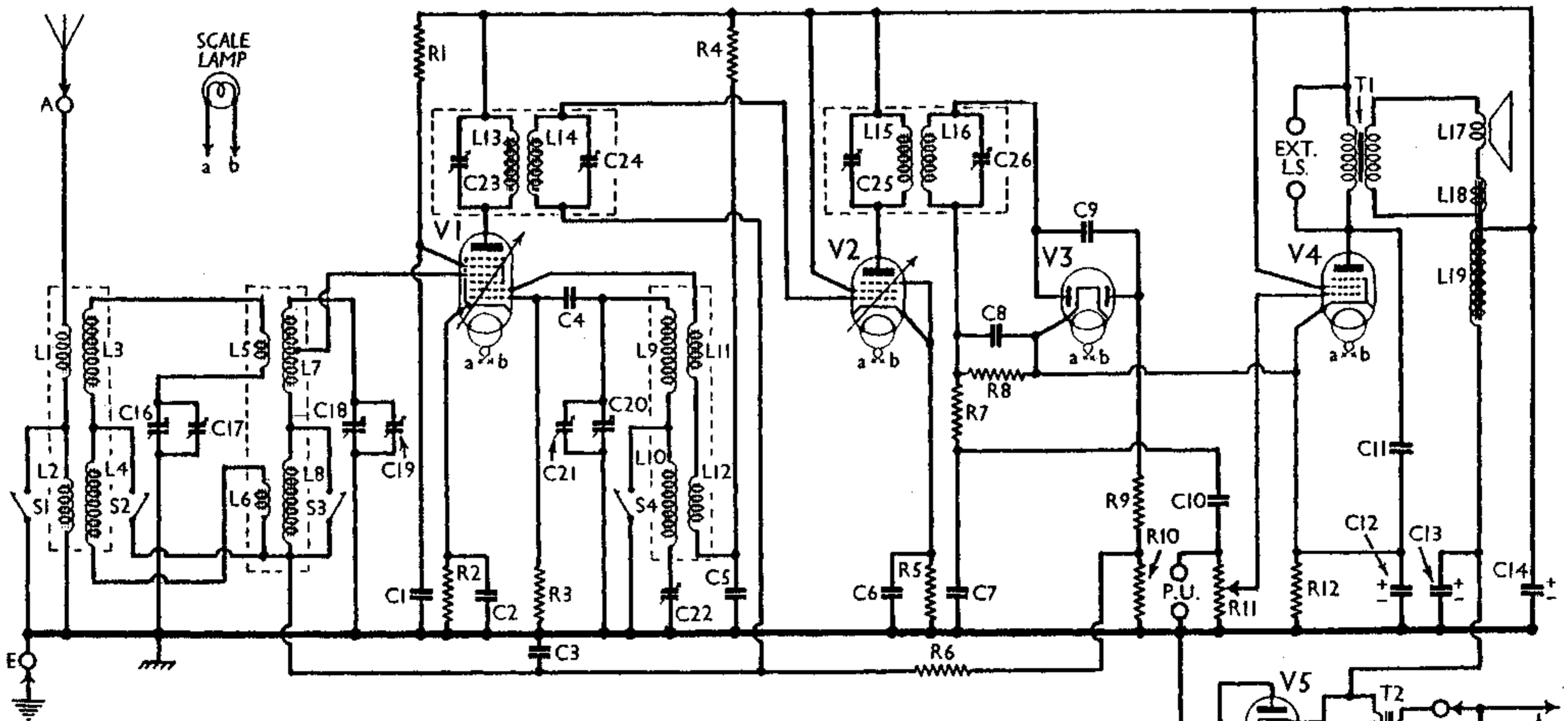
Circuit diagram of the Alba 540 A.C. superhet table model, and the 640 console. The 740 radiogram has a similar circuit, but with additions described under "Radiogram Modifications" on p. VIII. Note that all the coils are iron-cored. A simple circuit is used for tracking, with shaped vanes for C20, and a L.W. tracking condenser, C22.
