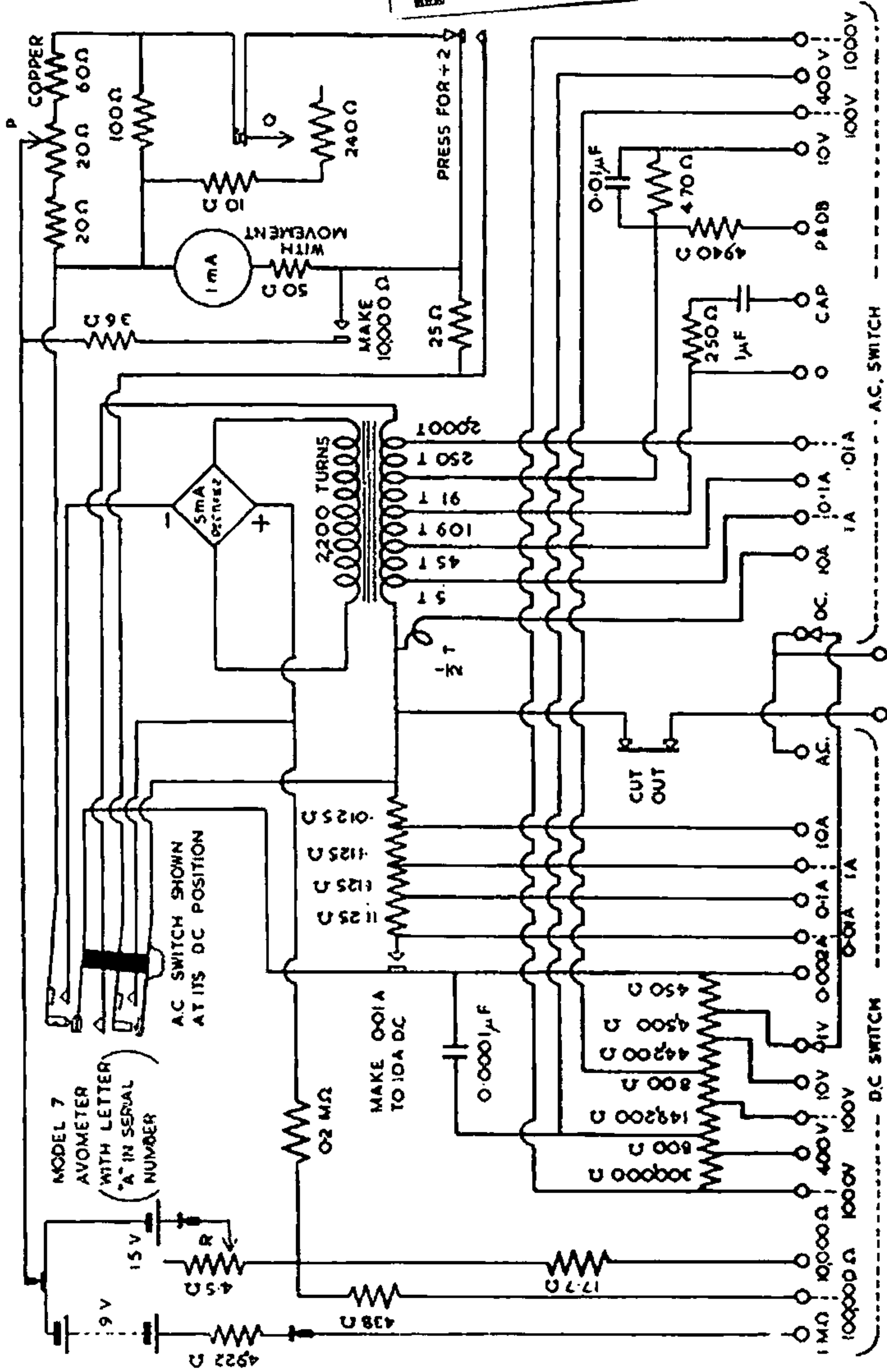
CIRCUIT DIAGRAM OF THE MODEL 7 AVOMETER
