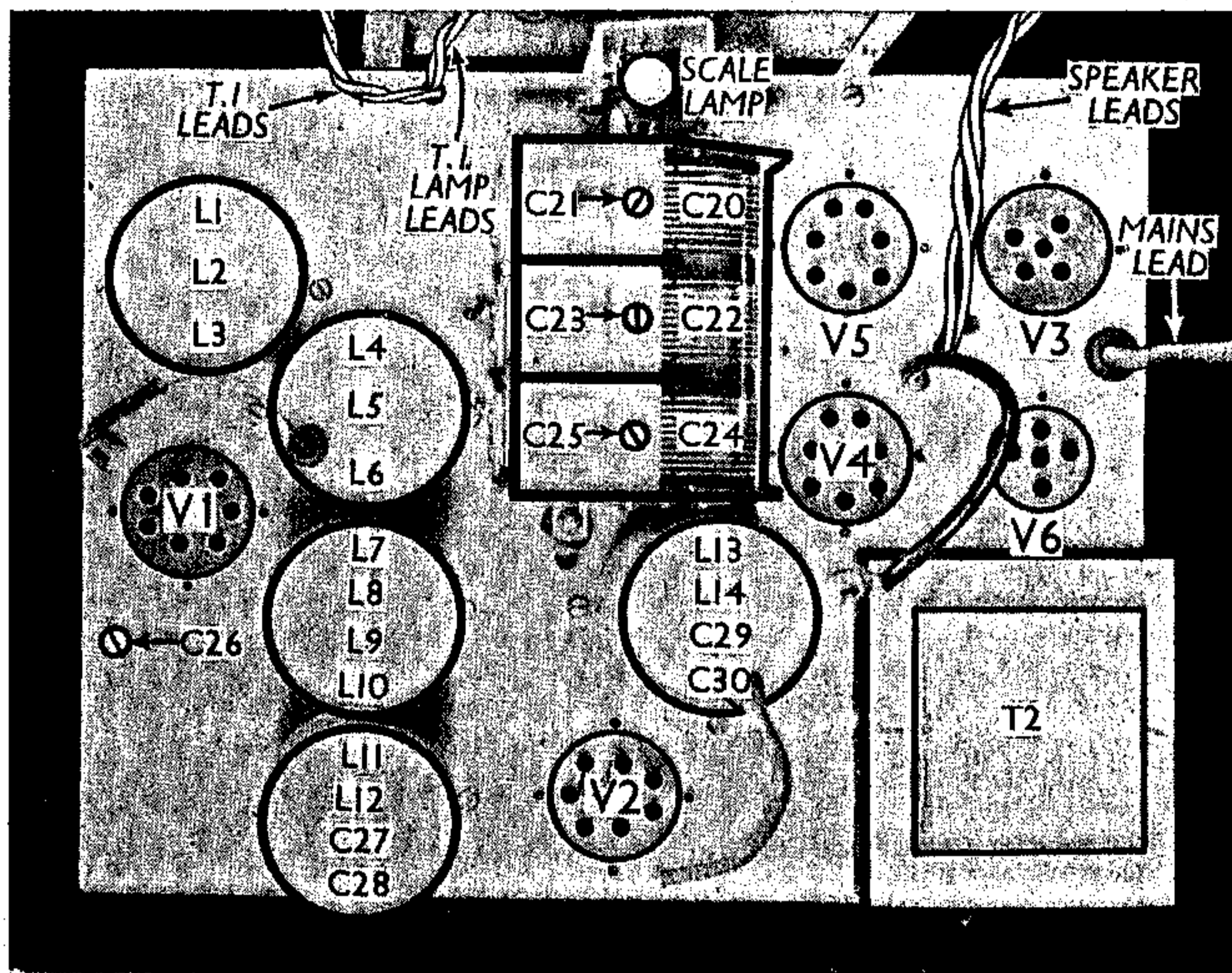
Plan view of the chassis. C26 is the variable part of the oscillator L.W. tracker. Note that the I.F. cans are not provided with holes through which the trimmers can be adjusted, since the latter are mounted at the base of each unit, and are adjusted from beneath the chassis.
